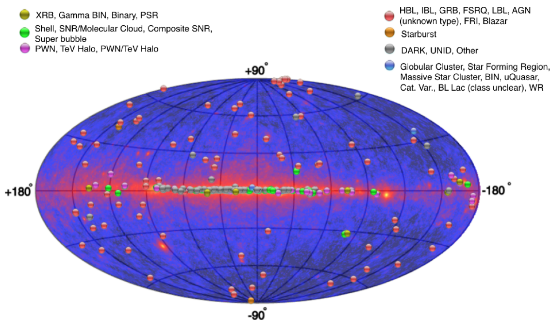
Figure 1.3: Catalog of TeV sources. From http://tevcat.uchicago.edu/
