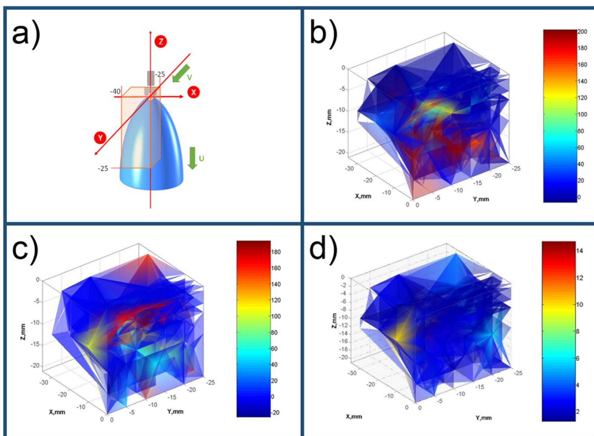
Figure 4.18. a) Schematic representation of the spray and the measurement zone. The measurement zone depends on x -, y - and z - positions set by the 3D axes table. The origin of the coordinate system is centered at the nozzle outlet position. Shown dimensions are (given in mm). b) Mean axial velocity U distribution in the first quarter of the spray (given in \text{ms}^{-1} ). c) Mean radial velocity V distribution in the first quarter of the spray (given in \text{ms}^{-1} ). d) Mean droplet size distribution in the first quarter of the spray (given in \mu\text{m} ).
