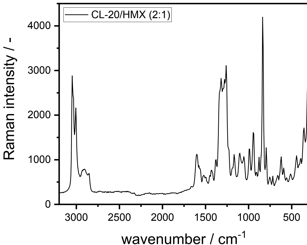
Figure 3.18. Raman spectrum of CL-20/HMX co-crystal (2:1) in a spectral range between 3200 \text{cm}^{-1} and 300 \text{cm}^{-1} .
