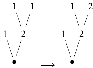
(b) The thick subtree from which it arose
