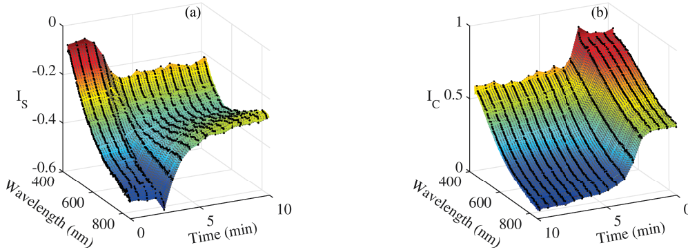
Figure 6.9 – Evolution of ellipsometric data (a) I_S and (b) I_C with deposition time during first 10 min of H_2 plasma treatment at 250 °C. The direction of time axis was reversed in case (b) to improve the visibility of I_C data.
