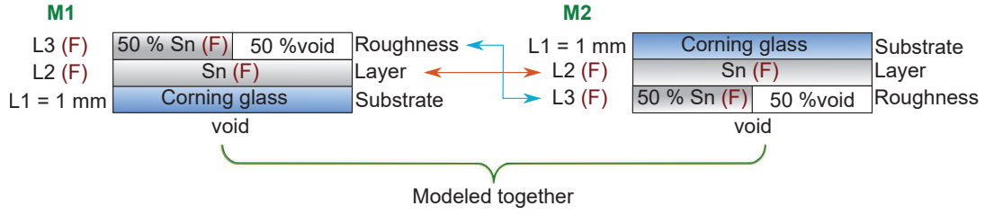
Figure 6.5 – Multi-layer optical models consisting of 1 mm Corning glass substrate ( L1 ), the Sn layer ( L2 ), and surface roughness ( L3 ) modeled by B-EMA containing 50 % of Sn and 50 % of void. Model M1 corresponds to the reference sample with Sn layer on top of Corning glass. Model M2 represents the same sample turned upside down. Red symbols F mark the free fitting parameters which are the thicknesses of layers L2 and L3 , and the optical function of Sn. Arrows mark the bound parameters.
