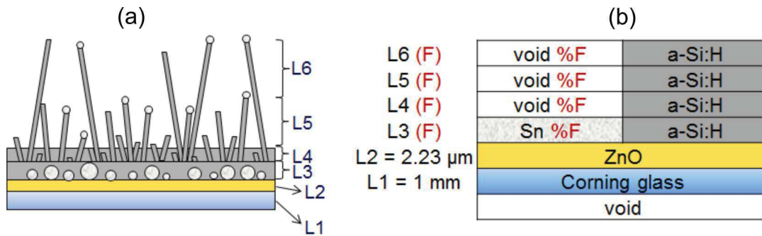
Figure 6.15 – (a) Schematic illustration of the first stages of silicon nanowire growth by the plasma-assisted VLS method using Sn droplets as the mediator for the growth. (b) Multi-layer optical model consisting of 1 mm Corning glass substrate ( L1 ), the aluminum doped ZnO layer of thickness of 2.23 \mu\text{m} ( L2 ), Sn droplets partially buried in the silicon represented by the B-EMA consisting of Sn, void, and silicon ( L3 ), the L4 layer formed by B-EMA of void and silicon representing short dense nanowires, and the L5 layer representing longer, less dense nanowires. Red symbols mark the free fitting parameters.
