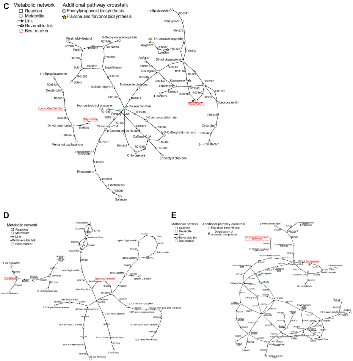
Fig. III.S4 | Metabolic networks. Best markers were mapped into a pre-existing A. thaliana metabolic network using MetExplore. A. Crosstalk between the sub-pathways “Starch and sucrose metabolism” and “Galactose metabolism”. B. Crosstalk between the sub-pathways “Cysteine and methionine derivatives”, “Arginine and proline derivatives” and “Alanine, aspartate and glutamate derivatives”. C. “Flavonoid biosynthesis” sub-pathway. D. “Carotenoid biosynthesis” sub-pathway. E. “Phenylpropanoid biosynthesis” sub-pathway. Adapted from Dussarrat et al., 2022, New Phytologist .
