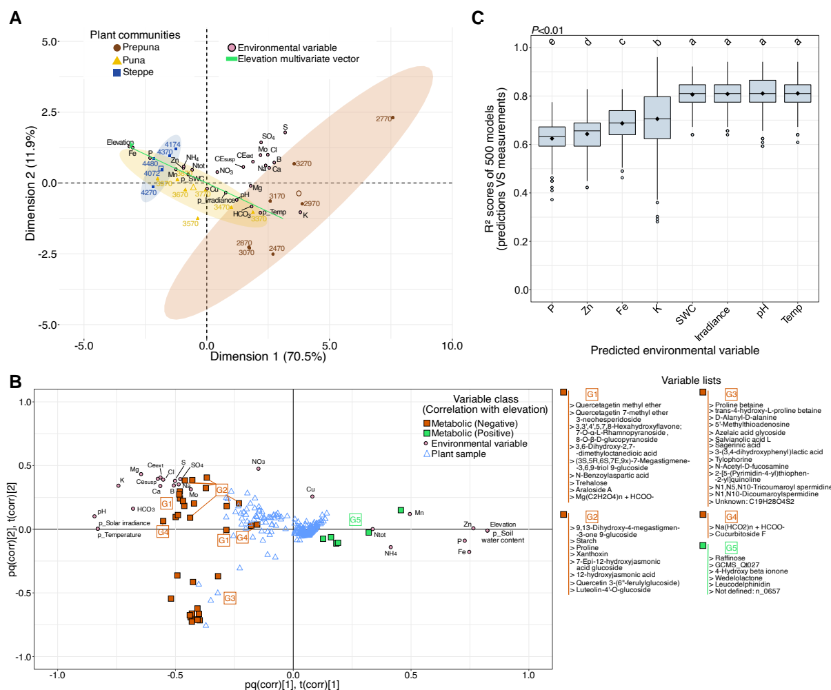
Fig. III.4 | Decomposition of the elevation factor and environment-metabolome covariation. A. Principal component analysis biplot. Discrimination of the sampling spots by the environmental data. SWC represents the soil water content while p_ represents a partially predicted parameter. B. Two-way orthogonal partial least squares describing the covariation between environmental and metabolic data. Hierarchical clustering analysis was realised with Pearson correlation and Ward algorithm. C. Boxplot showing the average R^2 scores (500 models) performed on the best discriminant environmental variables using the 66 best metabolic markers. Letters indicate statistical significance (Tukey's test, P < 0.01 ). Soil W cont represents the soil water content, Temp represents the temperature. The box in each box plot illustrates the lower, median and upper quartile values, and the vertical lines show the range of the R^2 variation in samples while squares and circles represent the mean R^2 and potential outliers, respectively. Adapted from Dussarrat et al., 2022, New Phytologist .
