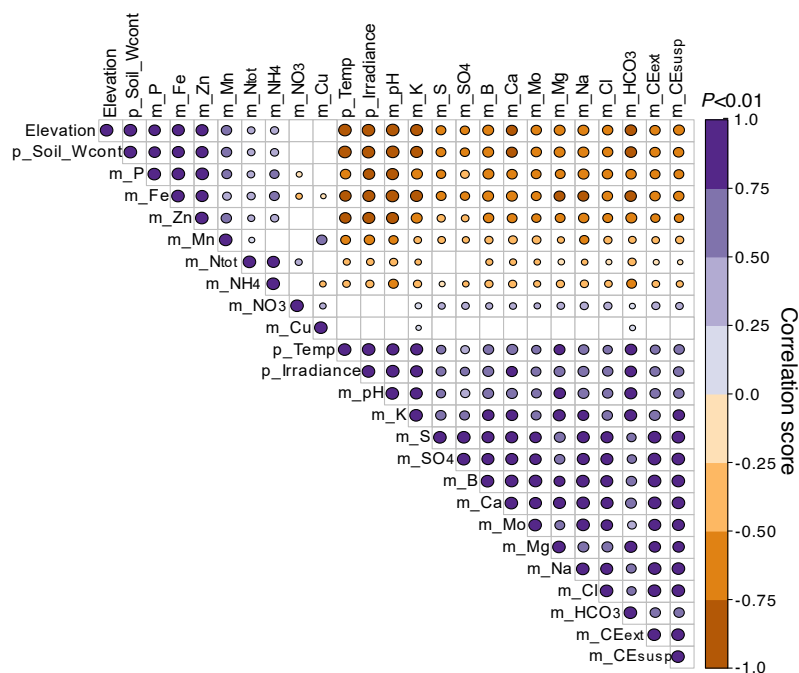
Fig. III.S6 | Decomposition of the elevation parameter. Correlation plot of the environmental data ( P < 0.01 , Pearson correlation). Adapted from Dussarrat et al., 2022, New Phytologist .
