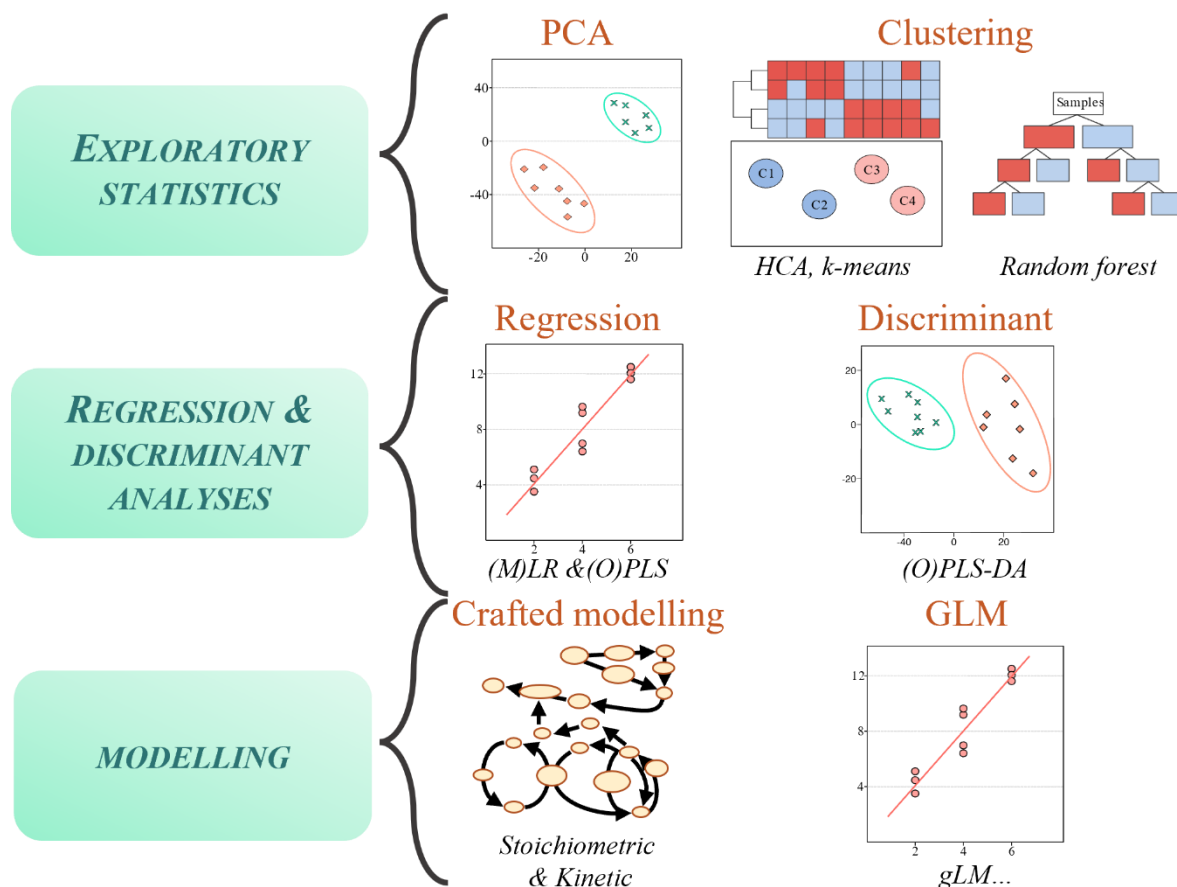
Fig. I.8 | Multivariate statistical analyses in untargeted metabolomics. PCA : principal component analysis, HCA : hierarchical clustering analysis, (M)LR : (multi) linear regression, (O)PLS : (orthogonal) partial least squares, DA : discriminant analysis, GLM : generalised linear modelling.
