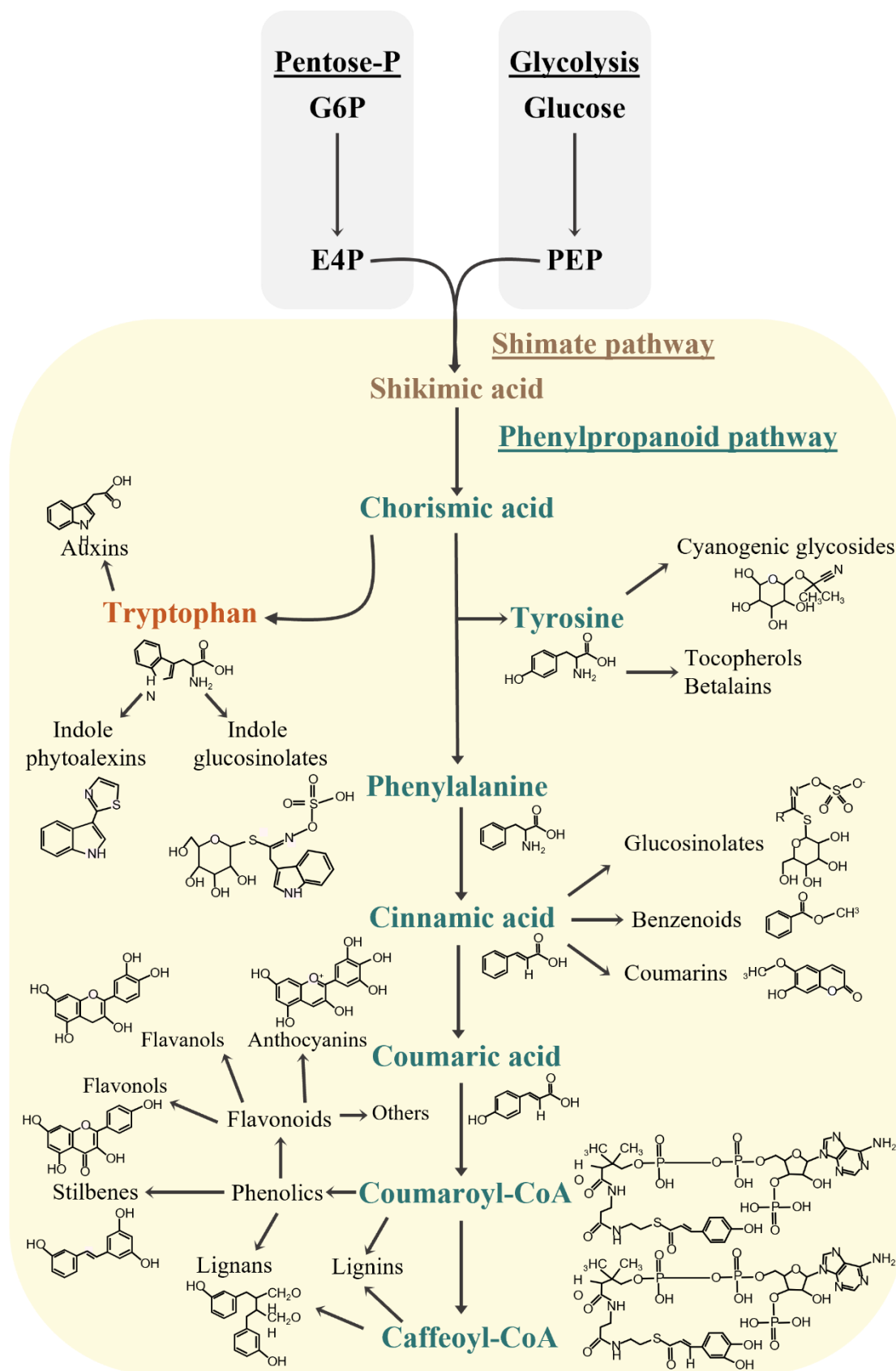
Fig. I.6 | Biosynthesis of polyphenols from shikimate pathway. G6P: glucose 6 phosphate, E4P: erythrose 4 phosphate, PEP: phosphoenol pyruvate.
