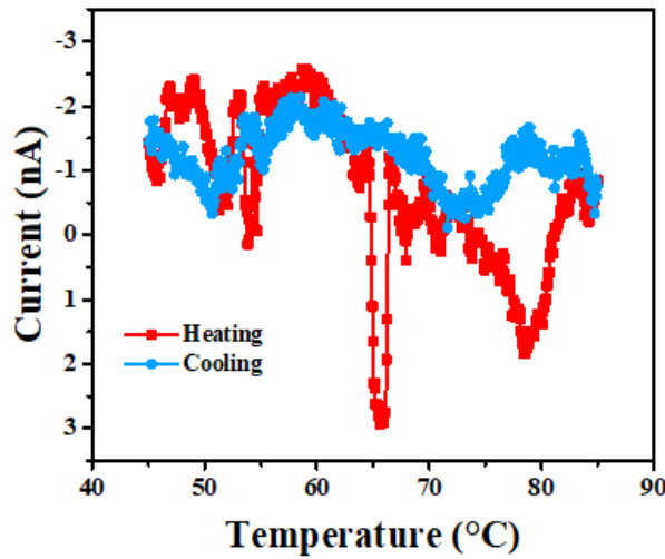
Figure 3.14: Representative temperature dependent current measurement for Device B. Measurement condition: V_G = -10 V, V_{DS} = -30 V, dT/dt = 5 °C/min. W = 50 \mu m, L = 1000 \mu m.
