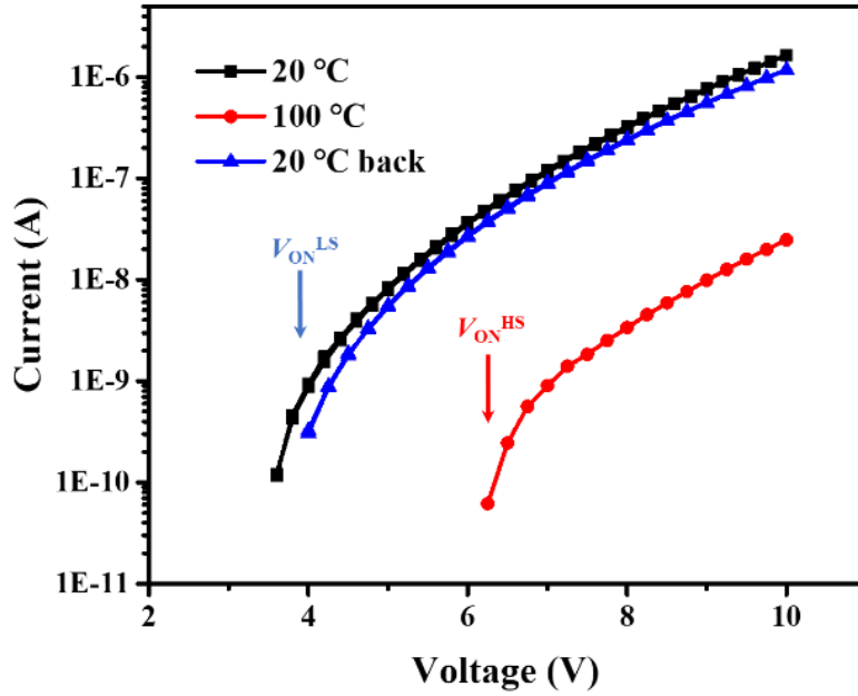
Fig 2.14: Log I - V representation of a ITO/100 nm [\text{Fe}(\text{HB}(\text{tz})_3)_2]/\text{Al} device characteristics at different temperatures evidencing a shift of the turn-on voltage ( V_{\text{ON}} ) between the LS and HS states.
