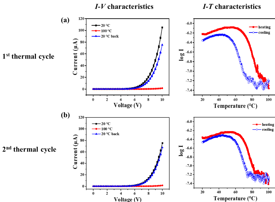
Figure 2.26: Electrical characteristics of an ITO/100 nm [\text{Fe}(\text{HB}(\text{tz})_3)_2] /Ca junction. The results of two successive thermal cycles are showed in (a) and (b). Left: I - V curves recorded at 20 °C and 100 °C and then again at 20 °C at rates of \pm 100 mV/s. Right: the \log I - T curves recorded with an applied bias of 5 V at scan rates of \pm 10 °C/min (a) and \pm 5 °C/min (b).
