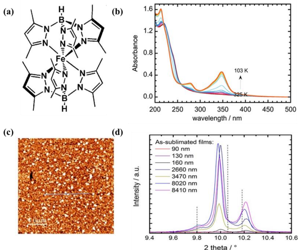
Figure 1.12: (a) Molecular structure of [\text{Fe}(\text{HB}(3,5\text{-(CH}_3)_2\text{pz)}_3)_2] . (b) UV absorption spectra recorded upon cooling the as-sublimed 130 nm-thick film. (c) AFM topography image of the as-sublimed 130 nm-thick film. (d) X-ray diffraction patterns of as-sublimed films between 90 and 8500 nm thickness [59].
