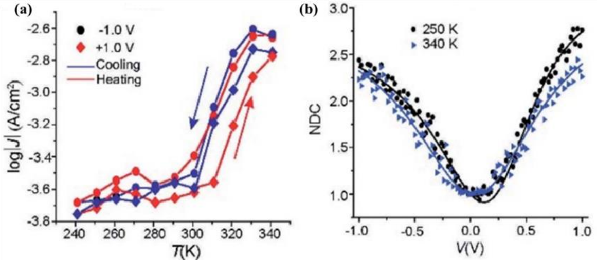
Figure 1.27: (a) Current density as a function of temperature at \pm 1.0 V applied bias. (b) Normalized differential conductance for a Cu/SLG/[Fe III (qsalI) 2 ]/NTf 2 /GaOx/EGaIn junction at different temperatures [78].
