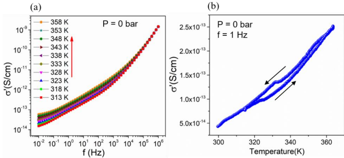
Figure 2.23: AC conductivity vs applied frequency for the bulk powder [Fe(HB(tz) 3 ) 2 ]. (a) Frequency dependence of the AC conductivity at various temperatures. (b) Temperature dependence of the AC complex conductivity at 1 Hz [58].
