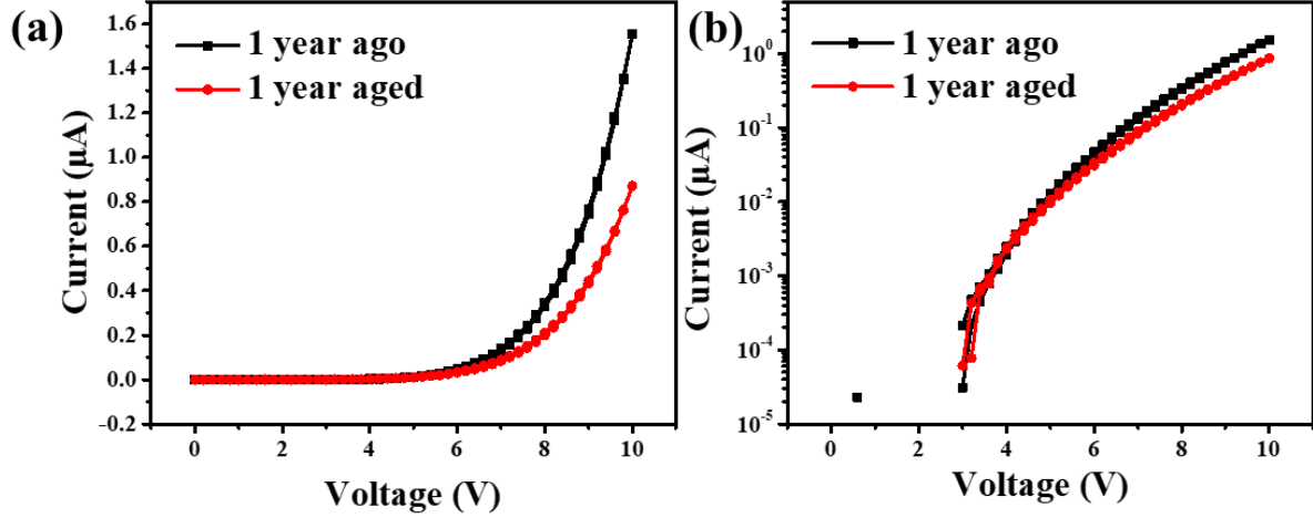
Figure 2.16: Room temperature I-V characteristics of a non-encapsulated ITO/100 nm [Fe(HB(tz) 3 ) 2 ]/Al junction just after fabrication and following 1 year storage in ambient conditions. Both linear (a) and logarithmic (b) representations are shown.
