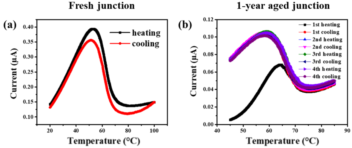
Figure 2.17: I-T characteristics of a non-encapsulated ITO/100 nm [Fe(HB(tz) 3 ) 2 ]/Al junction: (a) fresh (in the 2 nd thermal cycle) and (b) 1-year aged. The I-T curves were recorded with an applied bias of 5 V at scan rates of \pm 1 °C/min.
