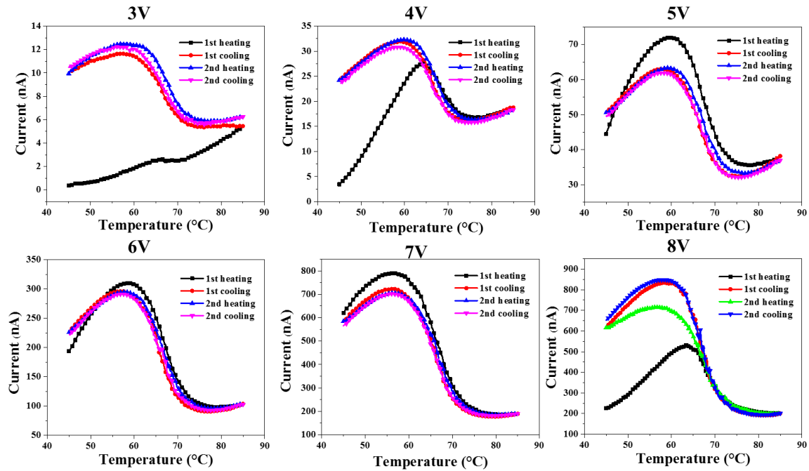
Figure 2.18: I-T characteristics of a “1-year aged” non-encapsulated ITO/100 nm [Fe(HB(tz) 3 ) 2 ]/Al junction. I-T curves were recorded with different applied bias between 3 and 8 V at scan rates of \pm 1 °C/min. For each bias, two successive heating-cooling cycles were carried out.
