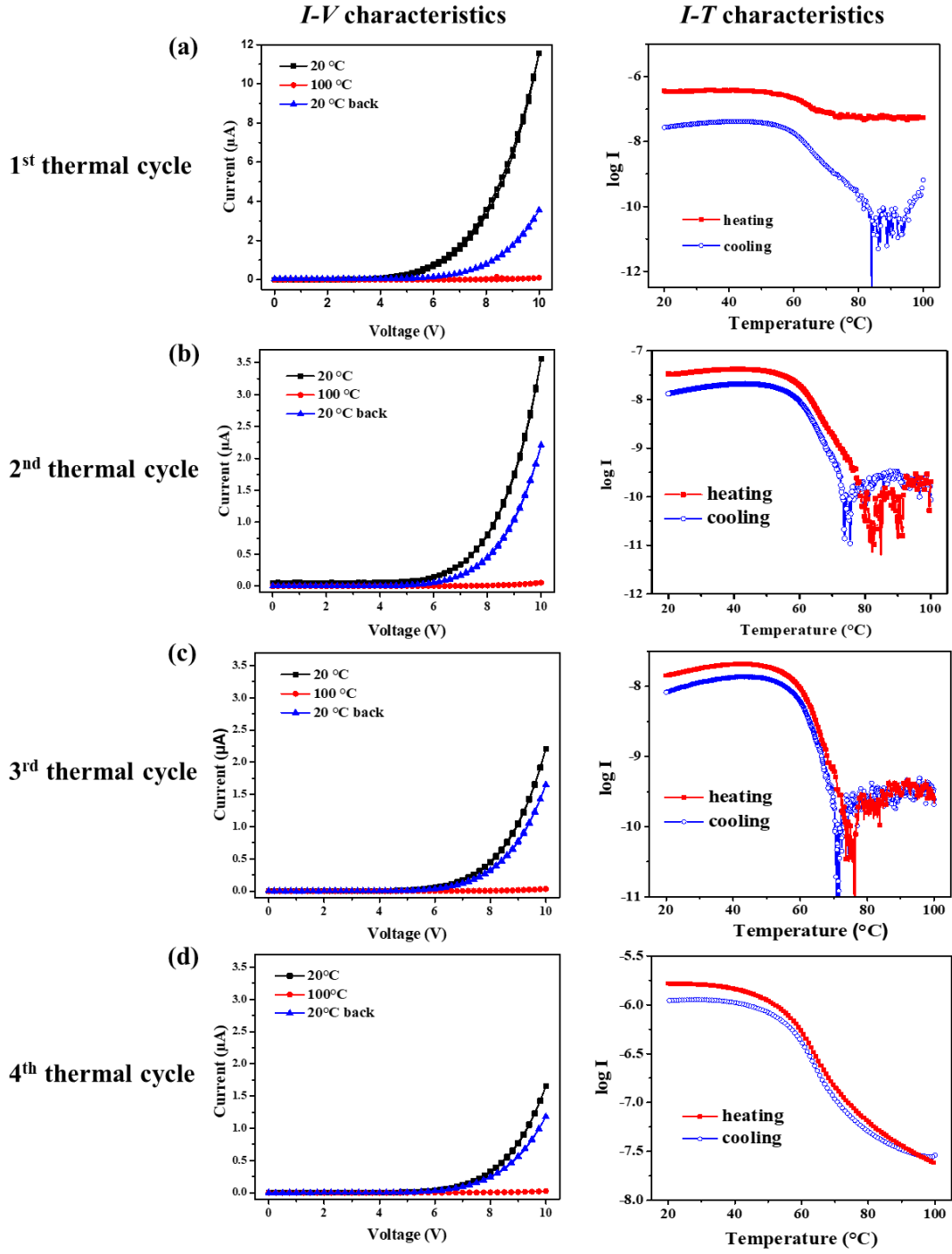
Figure 2.13: Electrical characteristics of an ITO/100 nm [\text{Fe}(\text{HB}(\text{tz})_3)_2]/\text{Al} junction. The results of four successive thermal cycles are showed in (a), (b), (c) and (d). Left: I - V curves recorded at 20 °C and 100 °C and then again at 20 °C at rates of \pm 100 mV/s. Right: \log I - T curves recorded with an applied bias of 5 V for first three thermal cycles (a, b and c, respectively) and 10 V for the forth thermal cycle (d), at scan rates of \pm 10 °C/min.
