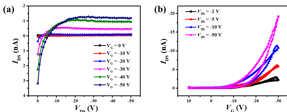
Figure 3.16: (a) Output characteristic ( V_G = 0, -10, -20, -30, -40 and -50 V) and (b) transfer characteristic ( V_{DS} = -2, -5, -10 and -50 V) of a ‘standard device’ measured at 45^\circ\text{C} . W = 70\ \mu\text{m} , L = 1000\ \mu\text{m} .
