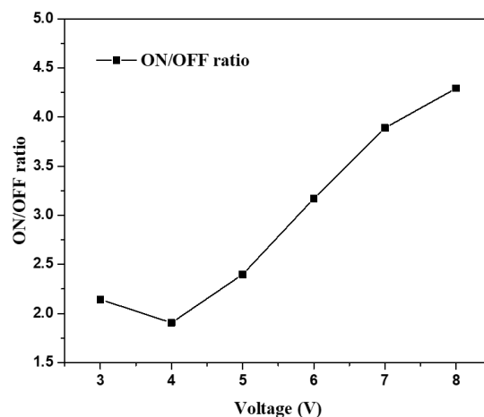
Figure 2.19: ON/OFF current switching ratio as a function of the applied bias voltage of a 1-year aged non-encapsulated ITO/100 nm [\text{Fe}(\text{HB}(\text{tz})_3)_2] /Al junction.
