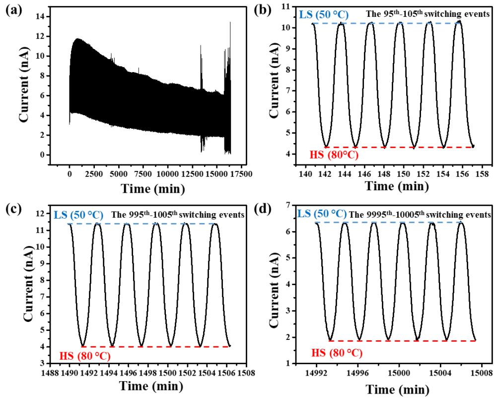
Figure 2.20: (a) Current switching cycles between the HS (low current intensity) and LS (high current intensity) states in a ITO/[Fe(HB(tz) 3 ) 2 ]/Al large-area vertical junction during >10,000 switches under a constant bias voltage of 3 V with a temperature ramping rate of \pm 20 °C/min range between 50 and 80 °C. Zooms are also shown on the 95 th – 105 th (b), the 995 th – 1005 th (c) and the 9995 th – 10005 th (d) switching events.
