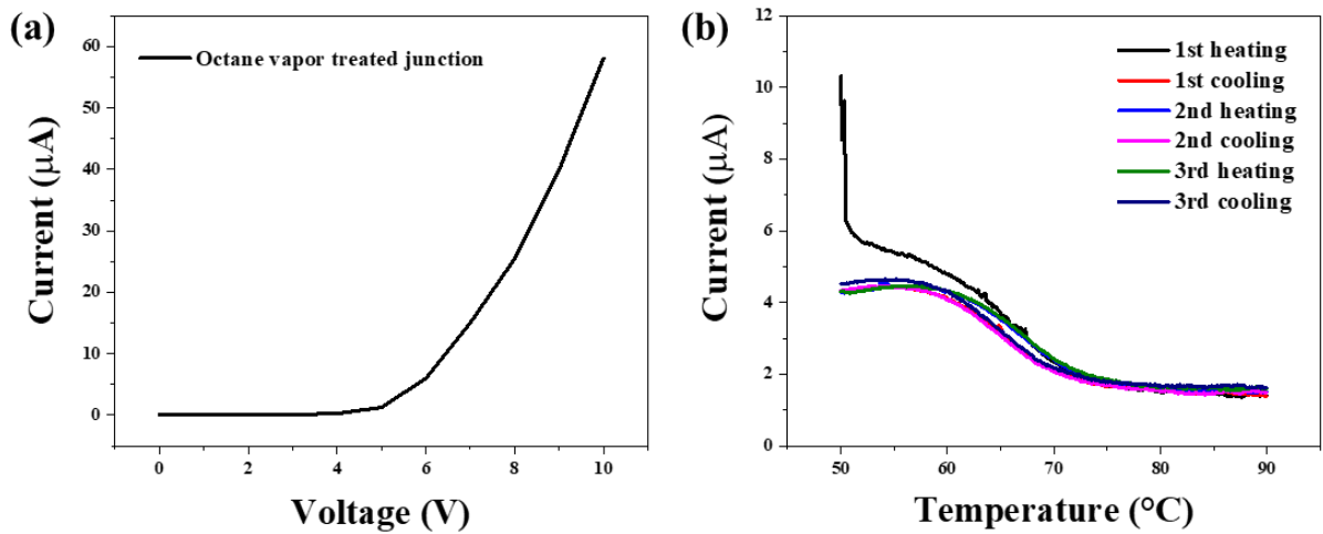
Figure 2.15: Electrical characteristics of an ITO/100 nm [\text{Fe}(\text{HB}(\text{tz})_3)_2] (octane vapor annealed)/Al junction. Left: I - V curve recorded at 20 ^{\circ}\text{C} at a rate of 100 mV/s. Right: I - T curves recorded under 8 V applied bias for the first three thermal cycles at scan rates of \pm 2 ^{\circ}\text{C}/\text{min} .
