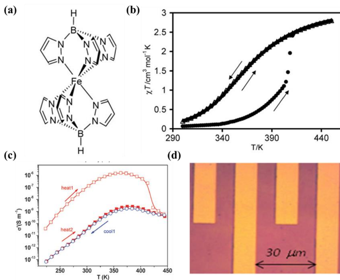
Figure 1.10: (a) Molecular structure of [\text{Fe}(\text{HB}(\text{pz})_3)_2] . Temperature dependence of the magnetic susceptibility (b) and ac conductivity (c) of the bulk. (d) Optical image of the thin film on interdigitated electrodes [55, 56].
