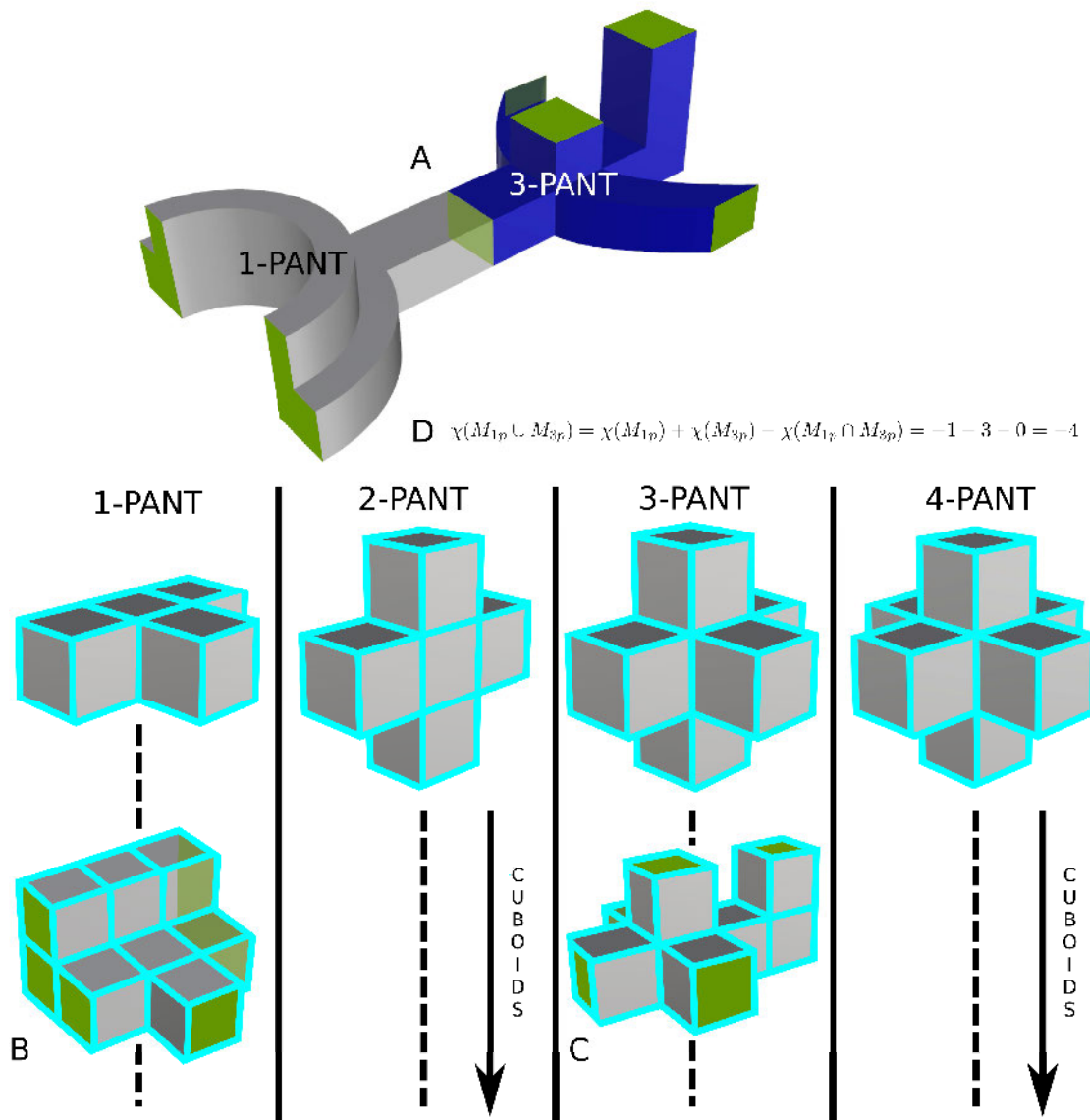
Figure 3.13: n -pant cuboids library. (A) A n -pant decomposition of an arbitrary B-Rep mesh M provided from CAD. (B) Adopted cuboid configuration \mathbb{C} chosen in the 1-pant column for the left part of (A). (C) Adopted cuboid configuration \mathbb{C} chosen in the 3-pant column for the right part of (A). Green surfaces represent cuboid faces which are mapped onto the boundaries of the M n -pant decomposition. (D) Euler characteristic of the n -pant topological decomposition (A) using union operator \cup .
