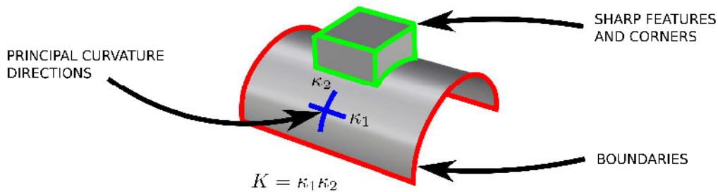
Figure 4.7: Relevant geometrical features which could be used for cross field interpolation. Sharp corners, boundaries and principal curvature directions refer to a certain global topological information embedded on the geometry. The Gauss-Bonnet theorem states the link between geometry and topology.
