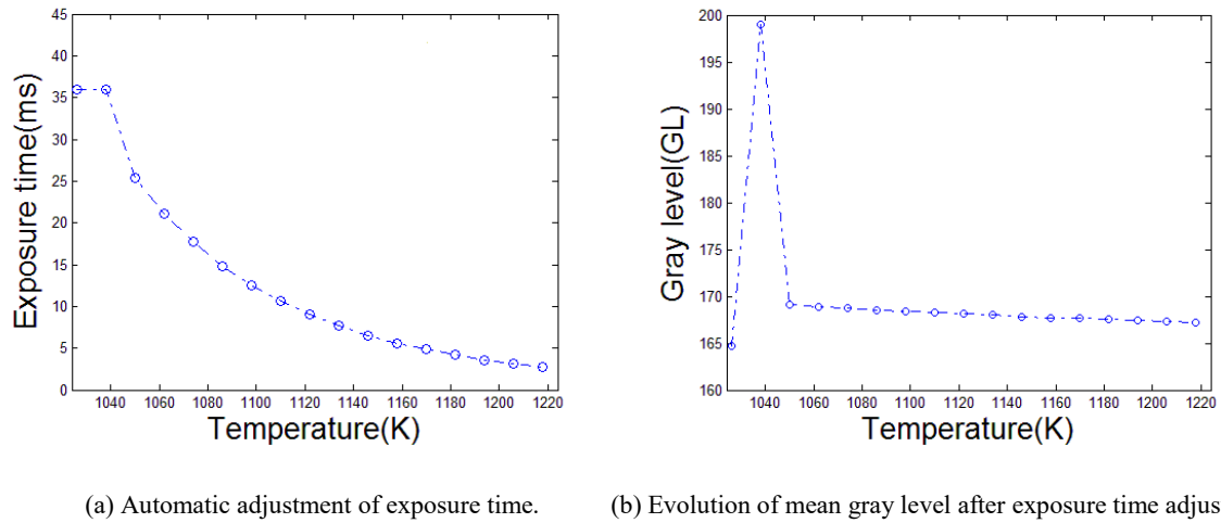
Fig. 2.10: Simulated results of linear algorithm.
