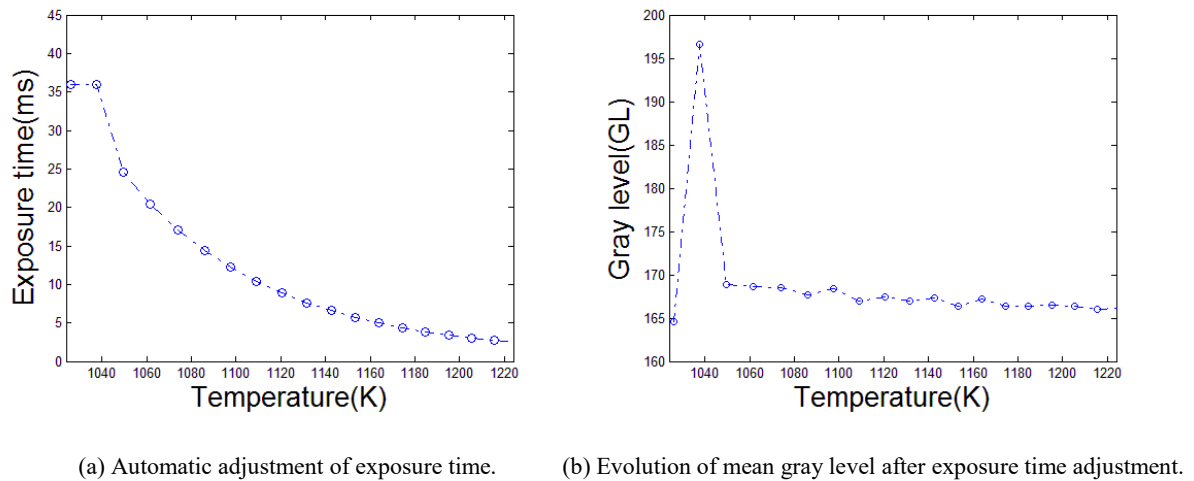
Fig. 2.11: Experimental results of linear algorithm.
