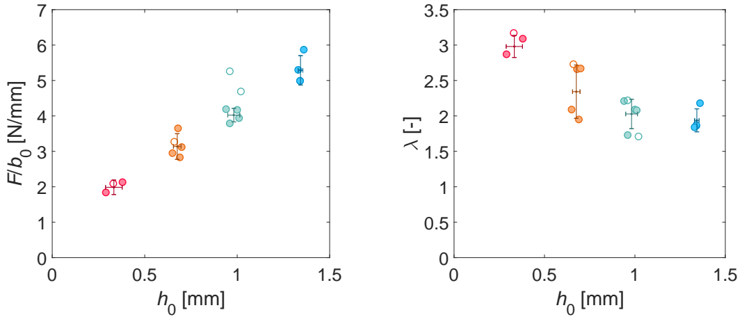
(a) Steady-state force normalized by the initial sample width b_0 .
