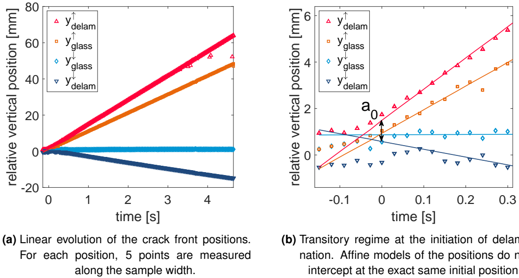
Figure II.11 Positions of delamination fronts and glass cracks over time in the TCTT.
