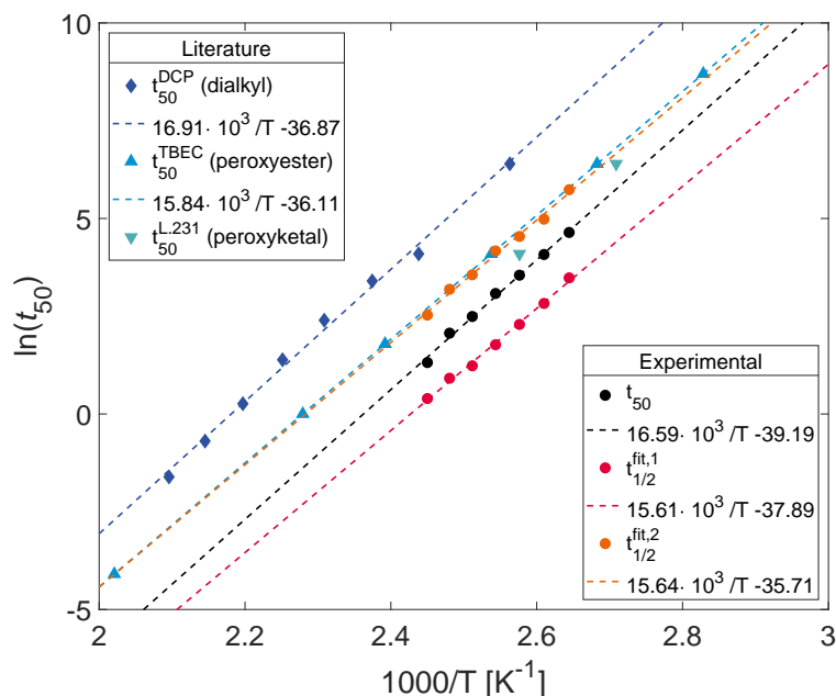
Figure IV.5 Arrhenius plots for the curing of the EVA interlayer. Literature data are taken from peroxides' technical information [89,91,92]
