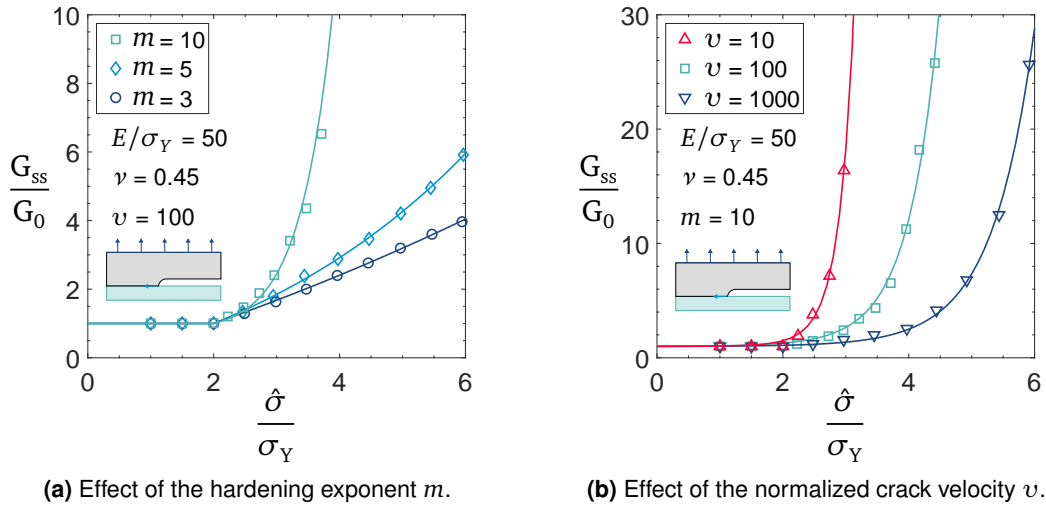
Figure VI.8 Steady state fracture energy vs. cohesive stress for a mode I adhesive crack, with a viscoplastic material.
