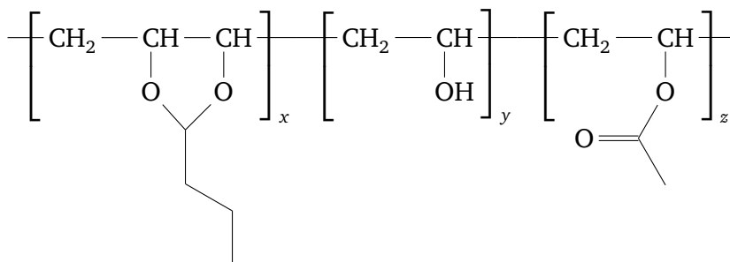
Figure II.1 PVB chemical formula ( x \approx 0.80 , y \approx 0.18 , z \approx 0.02 )
