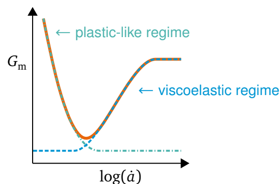
Figure VII.6 Combination of viscoelastic and plastic contribution to the work of fracture with PVB. The low-rate limit in the TCTT arises from plastic-like processes.
