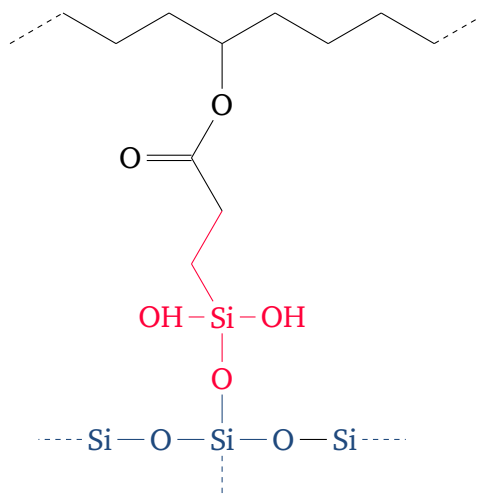
Figure II.5 Vinyltriethoxysilane binding the glass substrate and the EVA interlayer.
