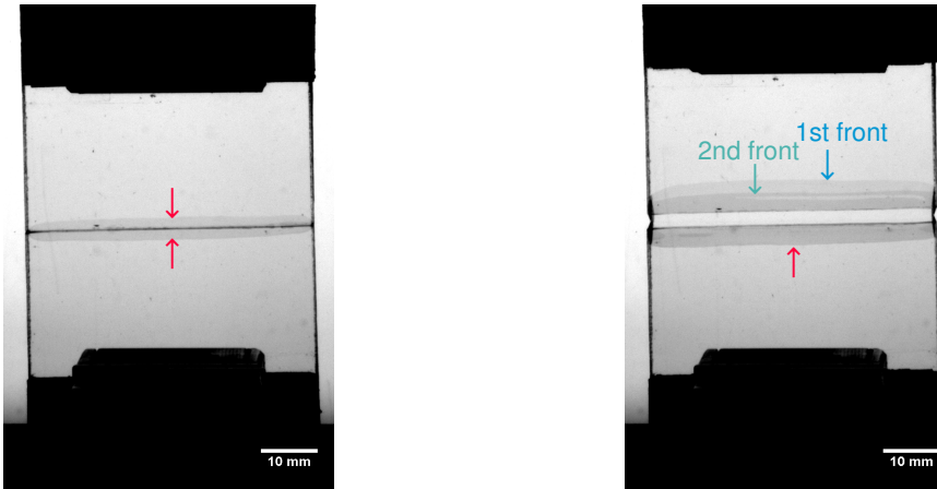
(a) \delta = 0.3 mm: the delamination fronts initiate only on one of the two glass faces.
