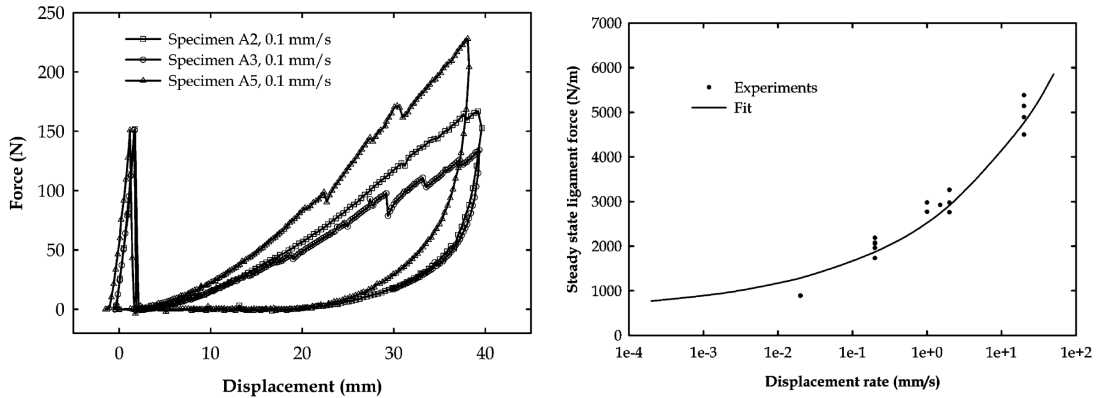
(a) Force vs displacement curves: the first peak corresponds to glass breakage, the following cycle to loading and unloading of the interlayer ligaments bridging the glass fragments.
