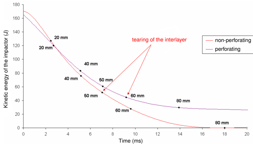
Figure I.3 Impactor kinetic energy decrease over time during a ball-drop-like impact, from Nourry 's PhD thesis [9] . The initial impactor energy is close to the critical energy for perforation. Lengths in mm correspond to the arrest distance of the impactor in the incremental procedure.
