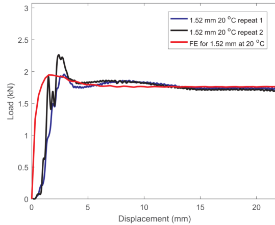
Figure VI.2 Force-displacement in the TCTT, fom Samieian.
