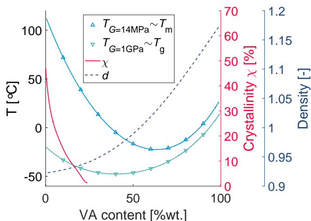
Figure II.4 EVA properties depending on the vinyl acetate (VA) weight content ( \bar{M}_n \sim 30,000 \text{ g}\cdot\text{mol}^{-1} ): melting temperature T_m , glass transition temperature T_g , crystalline content \chi and density d . Data were taken from Salyer & Kemyon [69] and re-plotted.
