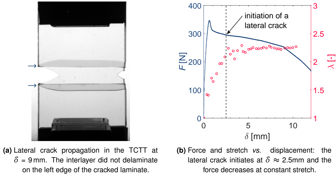
Figure III.4 Lateral crack initiation and propagation in the TCTT for the thinnest interlayer ( h_0 = 0.38 mm).
