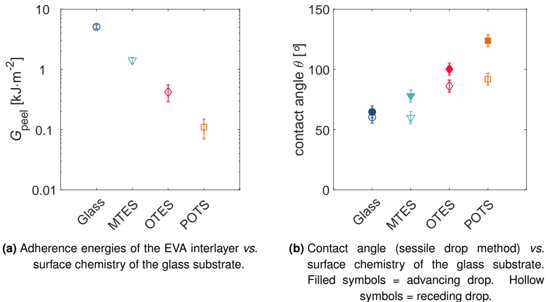
Figure V.2 Controlling adhesion of EVA via surface chemistry: peel adhesion and contact angle.
