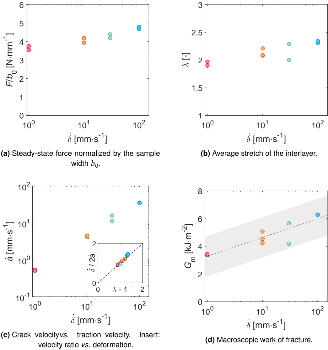
Figure V.8 Through Crack Tensile Test at varying traction velocities with EVA-laminates. T = 20^\circ\text{C} , initial interlayer thickness h_0 = 1\text{ mm} .
