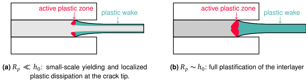
Figure V.7 Scenarios of plastic dissipation in the TCTT: (a) small-scale yielding vs. (b) development of the active plastic zone over the entire thickness of the interlayer.
