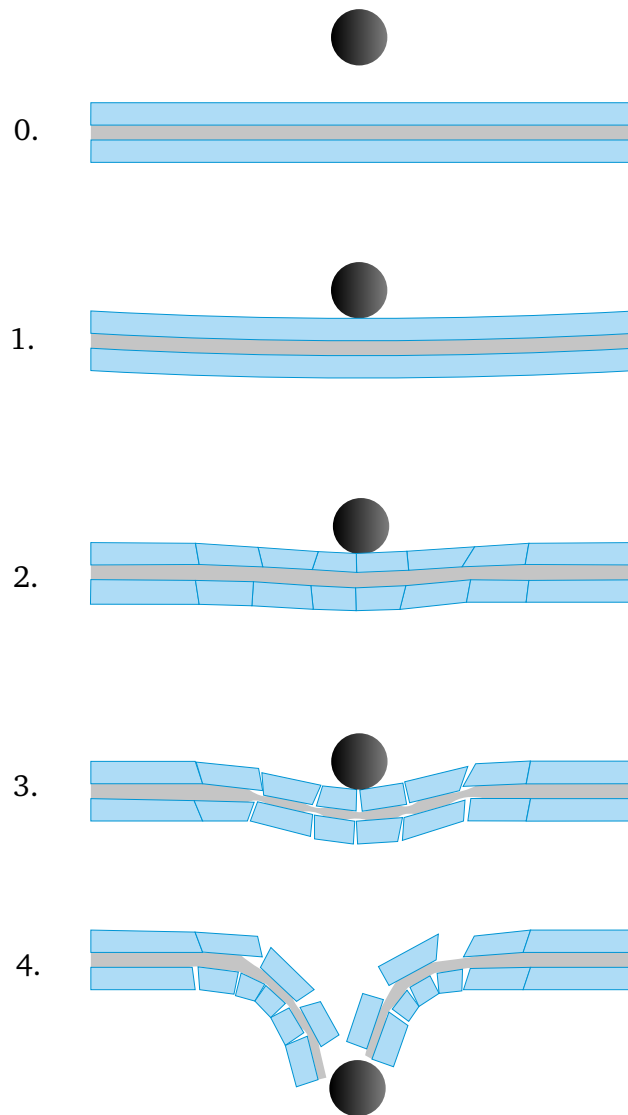
Figure I.2 Schematic of laminated glass during impact: 1. bending, 2. shattering, 3. stretching, 4. tearing and perforation.
