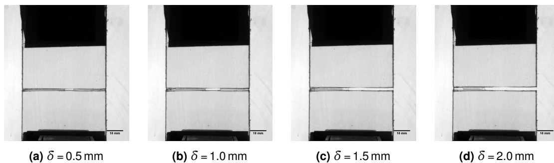
Figure V.1 Through Crack Tensile Test of an EVA laminate: immediate rupture
