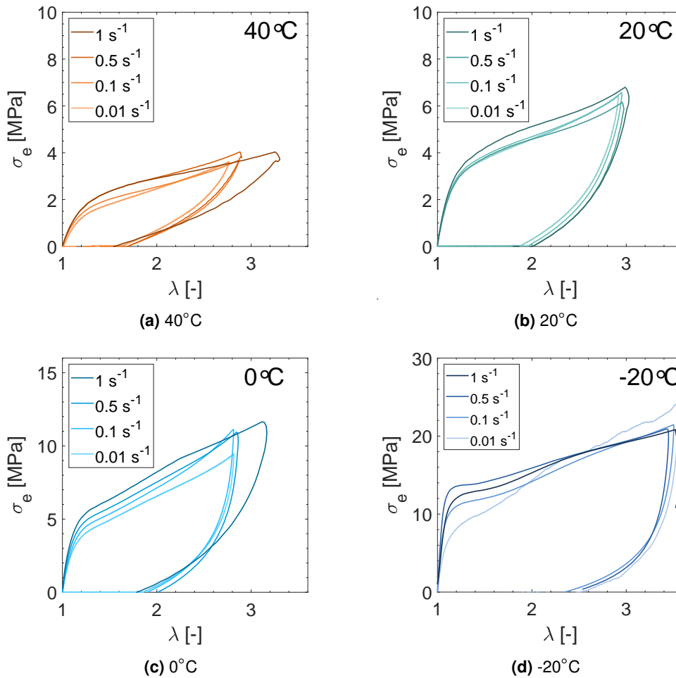
Figure IV.8 Engineering stress vs. stretch curves of EVA until 200% deformation at strain rates from 0.01 \text{ s}^{-1} to 1 \text{ s}^{-1} (maximal displacement = 50 mm).
