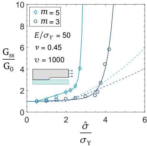
(a) Fracture energy vs. cohesive stress: effect of the plastic exponent m . Results in mode I are plotted in dashed lines.
