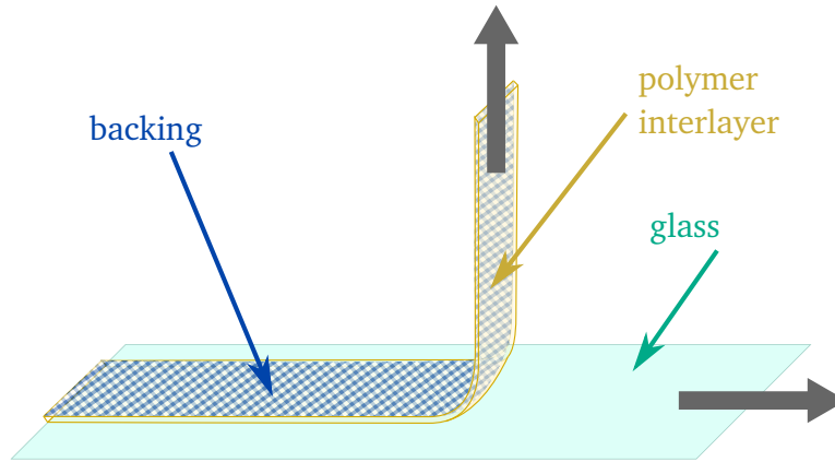
Figure II.9 Schematic of the peel sample and peel test geometry
