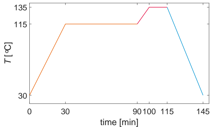
Figure IV.1 Thermal cycle for EVA lamination
