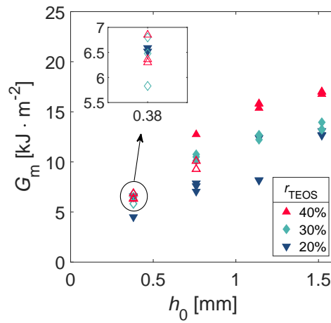
Figure III.10 Experimental macroscopic work of fracture. Filled symbols: steady-state delamination. Hollow symbols: interlayer rupture after partial delamination.
