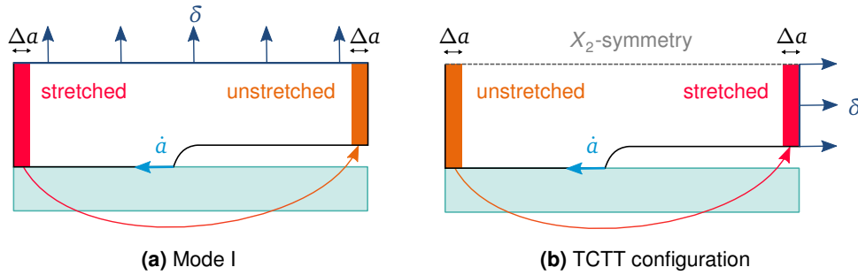
Figure VI.7 Energy release rate calculation in steady-state configuration. The energy required to propagate the crack by a length \Delta a is equal to the difference in stored energy \Delta U between the unstretched and stretched strips.
