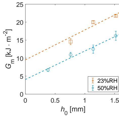
Figure III.12 Macroscopic work of fracture for two relative humidities. Data at 50%RH were from Elzière [4] .
