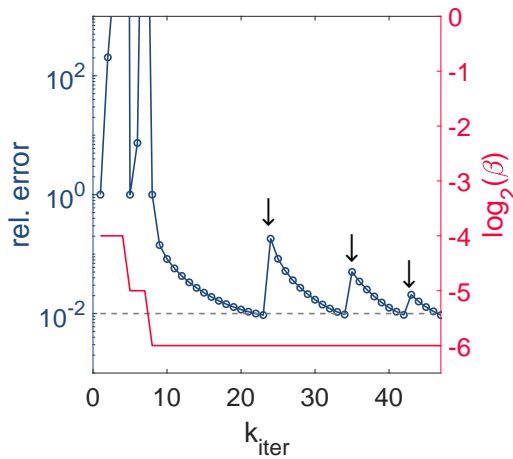
Figure A.4 Convergence plot: relative error vs. iteration number.
