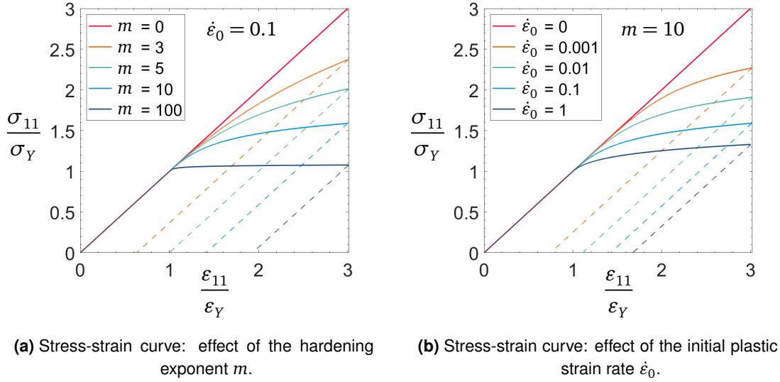
Figure VI.3 Uniaxial extension response of the viscoplastic material, at imposed stress rate.
