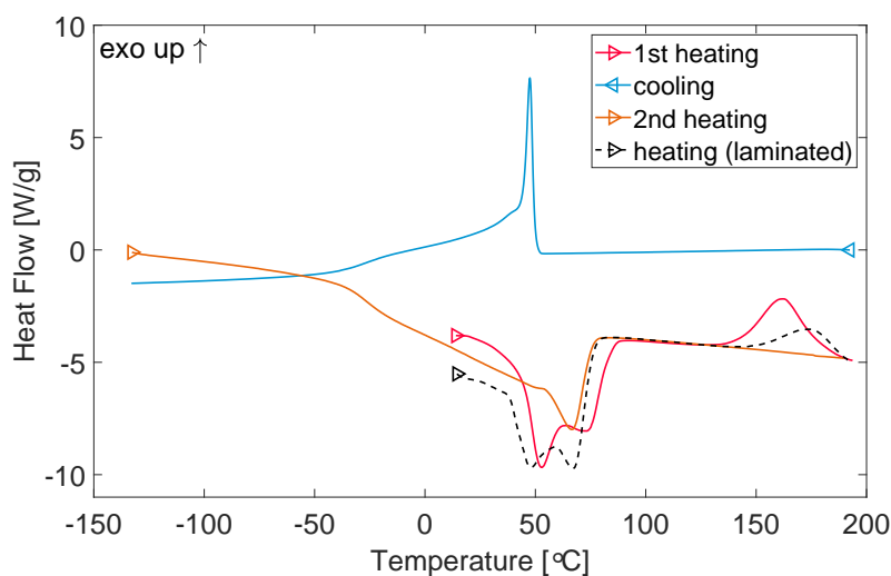
Figure IV.2 DSC of the EVA interlayer. Solid lines: pristine EVA in a heat-cool-heat cycle (heating rate = 20^{\circ}\text{C}\cdot\text{min}^{-1} , cooling rate = 10^{\circ}\text{C}\cdot\text{min}^{-1} ). Dashed line: EVA after lamination between glass plies.
