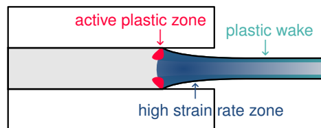
Figure V.11 Elasto-visco-plastic case: viscous dissipation in the high-strain rate zone over the entire thickness of the interlayer.
