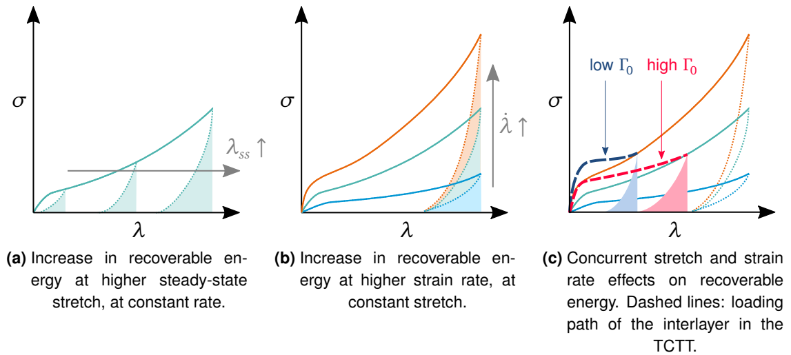
Figure III.13 Schematic of the evolution of the elastic recoverable energy in PVB.
