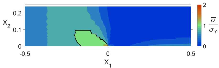
(a) Equivalent stress \bar{\sigma} . Black line: limit of the active plastic zone.
