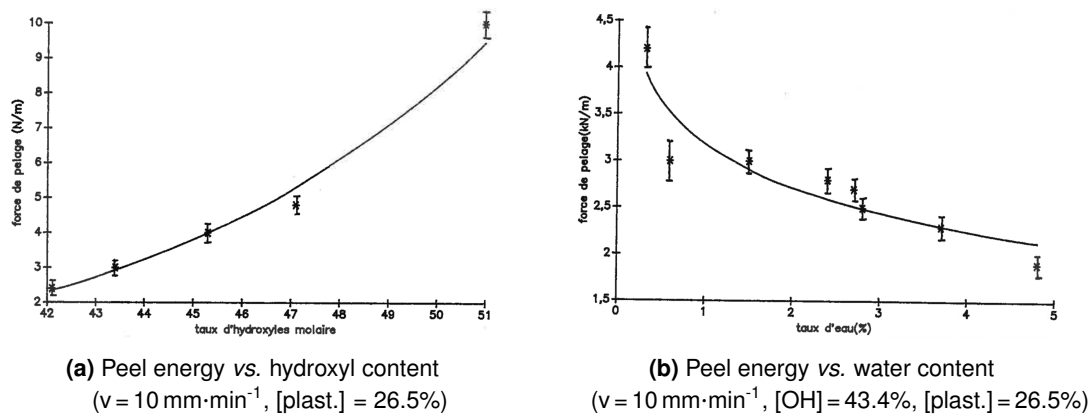
Figure I.7 Effects of the hydroxyl content [OH] and the water content on the adhesion of plasticized PVB, with a plasticizer content [plast.] = 26.5%, from Klock's PhD thesis [29]
