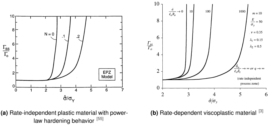
Figure I.14 Ratio between steady-state fracture energy and cohesive energy, as a function of the ratio between cohesive stress and yield stress. (a) Rate-independent plastic material, (b) rate-dependent viscoplastic material.
