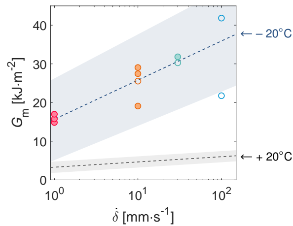
(c) Macroscopic work of fracture G_m vs. traction velocity \dot{\delta} . Shaded areas: 95% prediction bounds of the linear models.
