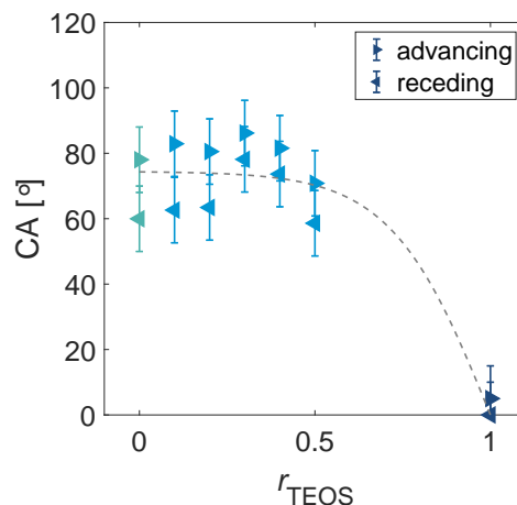
Figure III.1 Contact angle between water and the glass substrate vs. TEOS content of the surface treatment. The grey dashed line is a guide for the eye.
