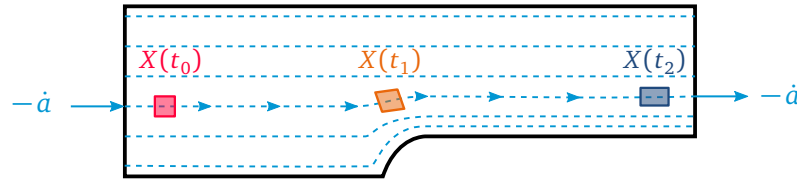
Figure VI.6 Time and space equivalence in steady-state Eulerian framework: the material element is translated along a material trajectory or streamline. Mechanical history, from t_0 to t_2 > t_1 > t_0 , is retrieved from the elements along the streamline.
