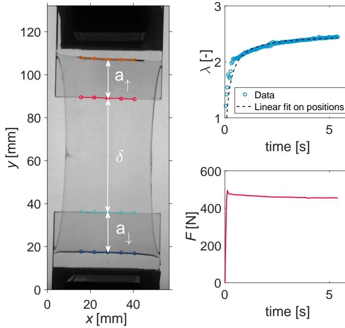
Figure II.12 Through Crack Tensile Test data analysis: measurement of the stretch by image analysis. Steady-state regime is reached when both force and stretch are constant with time.
