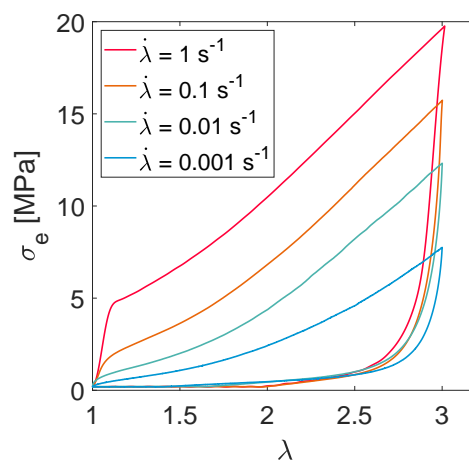
Figure II.2 Uniaxial tensile test on PVB: engineering stress vs stretch.
