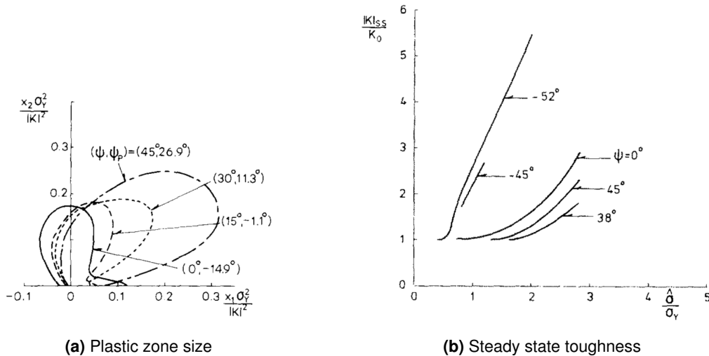
Figure I.15 Effect of mode mixity on the fracture toughness in a plastic material, from Tvergaard & Hutchinson [54]
