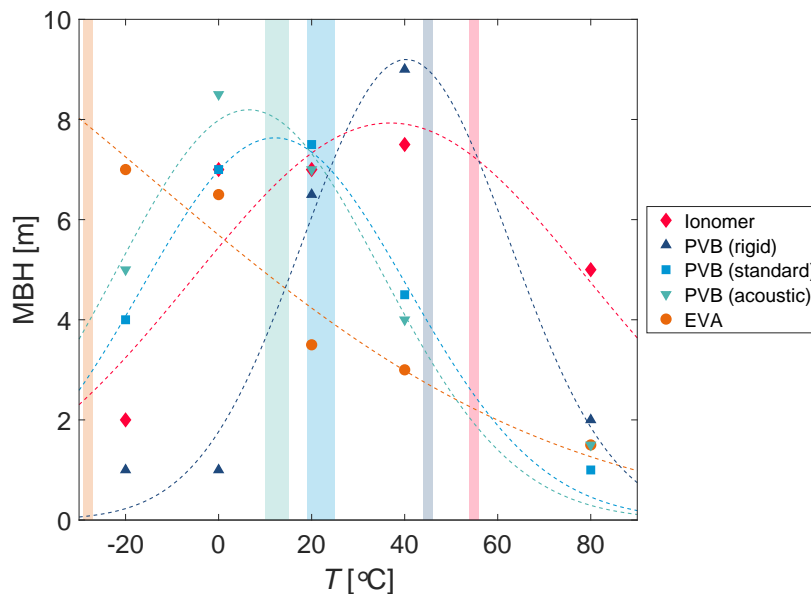
Figure I.4 Mean Break Height of laminates made of different interlayers, measured at temperatures from -20^{\circ}\text{C} to 80^{\circ}\text{C} . Dashed lines are gaussian fits made to highlight the optimum of performance. Shaded bars indicate the glass transition temperature of each polymer. Data from Novotny & Poot (2016) [12]
