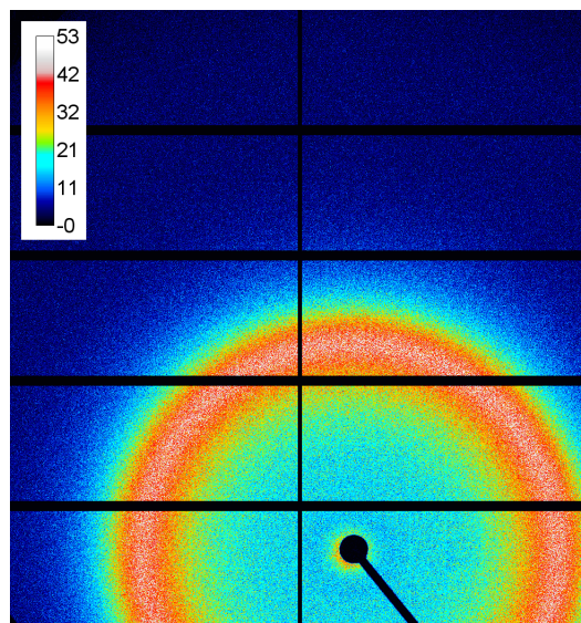
Figure II.7 Wide angle X-ray scattering of PVB. Color bar = photon count N .
