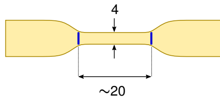
Figure II.8 Schematic of a tensile specimen. Paint marks are applied for video extensometry measurements. Dimensions are in mm.
