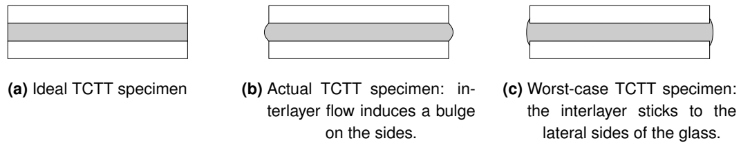
Figure III.5 Schematics of a TCTT specimen, view through the width. Lamination conditions (heat, pressure, sealing) may induce the formation of a bulge at the edges of the sample.
