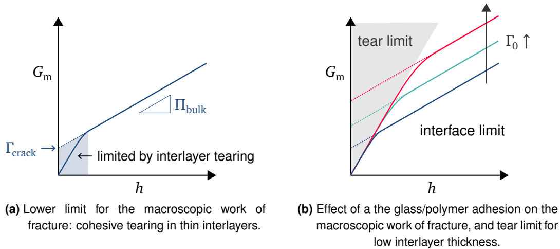
Figure VII.2 “Rupture” limit in the TCTT for thin interlayers
