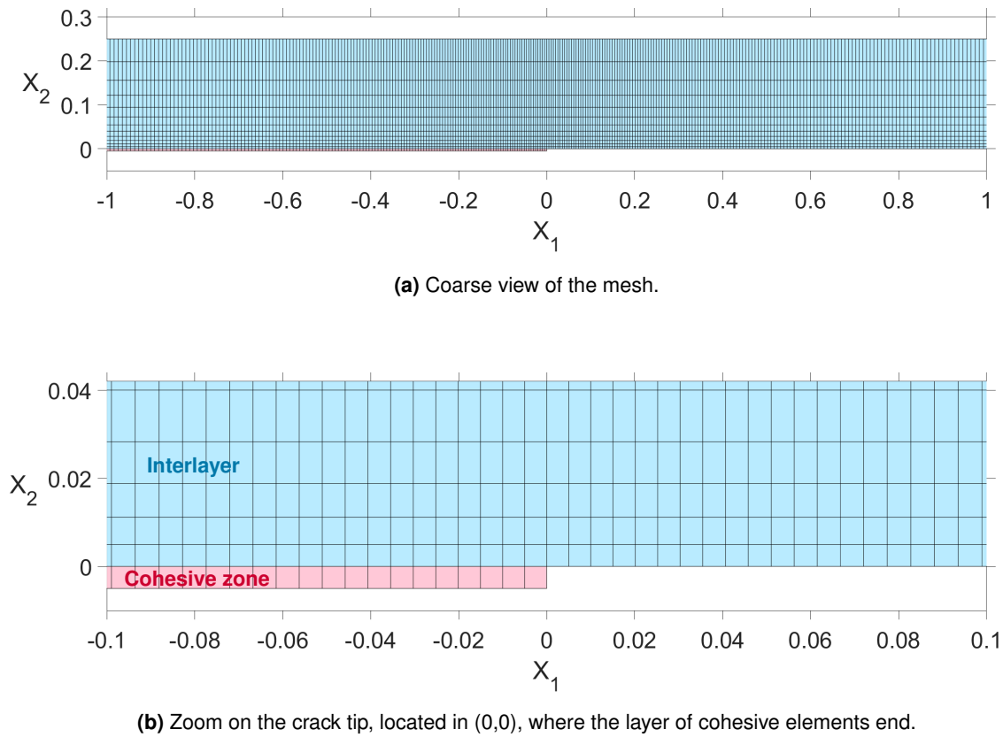
Figure A.1 Finite element mesh obtained with graded edge seeding and the advancing front algorithm in ABAQUS.
