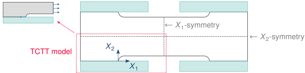
Figure VI.4 Steady-state model of the TCTT: the X_1 -axis and X_2 -axis symmetries allow to model only one quarter of the model.
