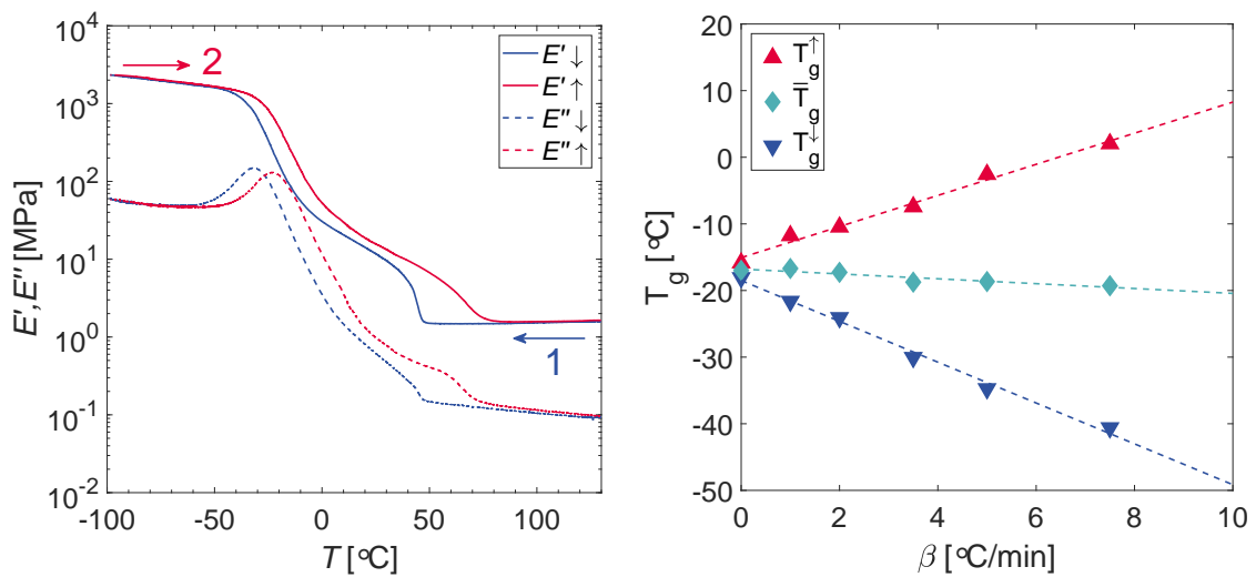
(a) Storage modulus E' and loss modulus E'' of EVA vs. temperature, 0.1% deformation, 1Hz. (heating/cooling rate \beta = 1^\circ\text{C}\cdot\text{min}^{-1} )
