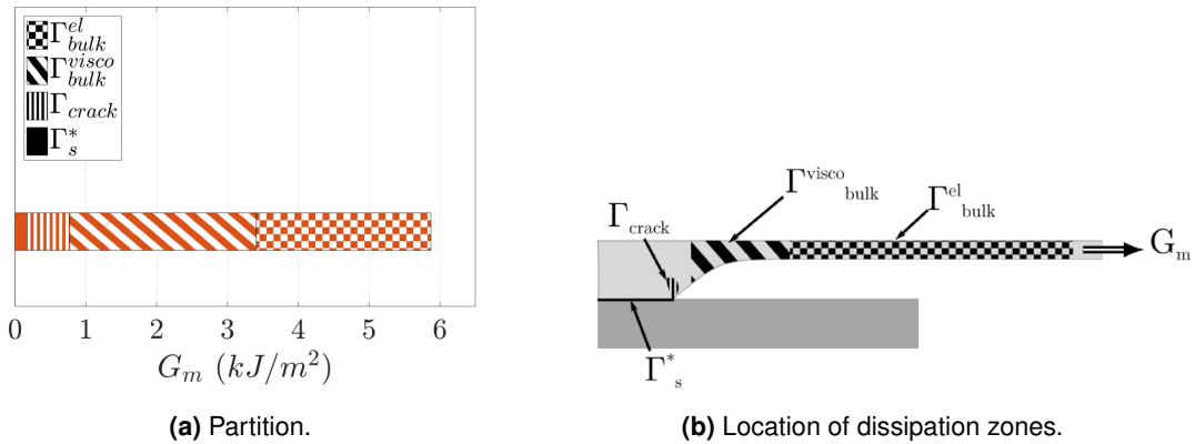
Figure VI.1 Macroscopic work of fracture, from Elzière.
