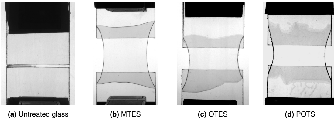
Figure V.4 Through Crack Tensile Test of EVA for various surface chemistries. ( T = 20^{\circ}\text{C} , \dot{\delta} = 10 \text{ mm}\cdot\text{s}^{-1} )
