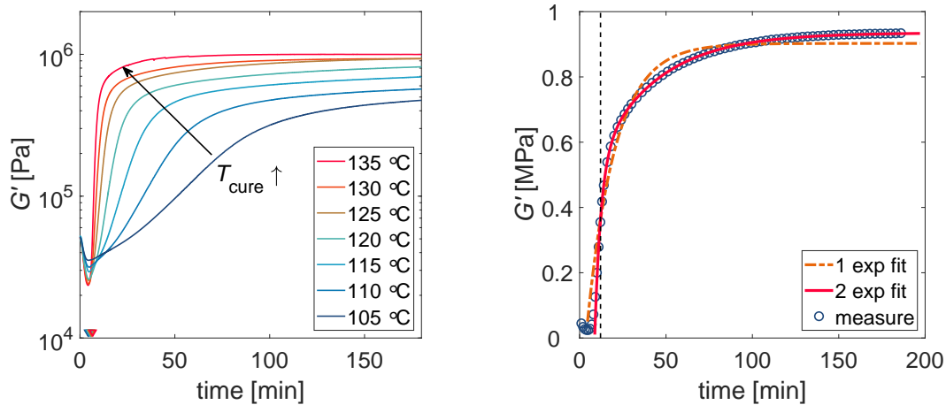
(a) Experimental cure laws G'(t) at various temperatures. The initial drop of G' is due to the heating from T_{init} = 90^\circ\text{C} to T_{cure} . Triangular markers indicate the time when T = T_{cure} .
