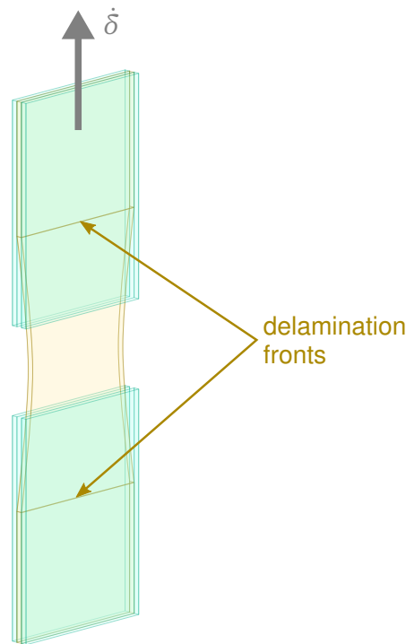
Figure II.10 Schematic of a Through Crack Tensile Test specimen during the test.
