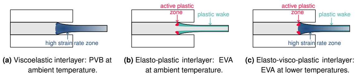
Figure VII.5 Schematic of the mechanisms for energy dissipation upon delamination and stretching of interlayers.
