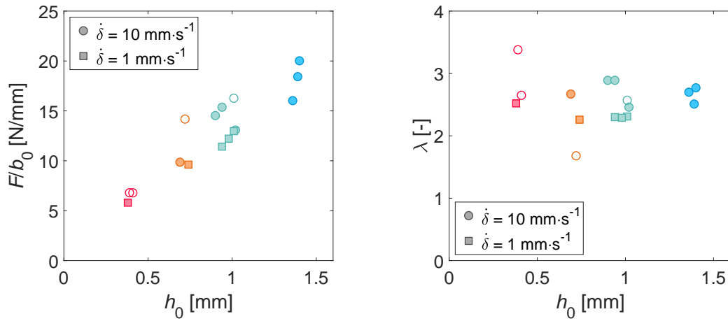
(a) Normalized delamination force.
