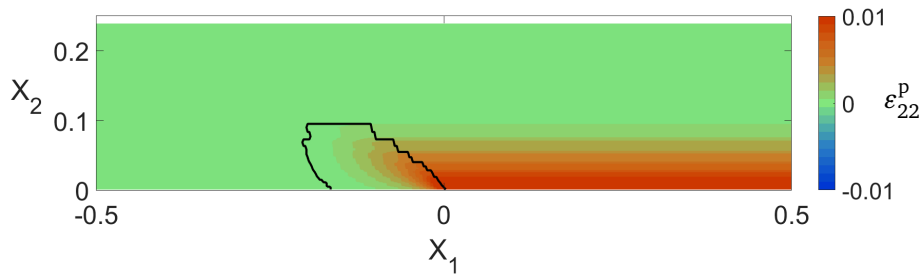
(b) Plastic strain \epsilon_{22}^p . Black line: limit of the active plastic zone.
