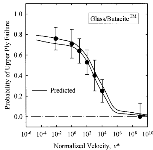
Figure I.5 Probability of upper glass ply failure vs velocity in biaxial flexure, from Bennison et al. [19]
