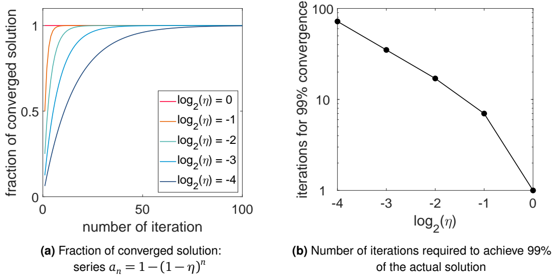
Figure A.3 Reduced-stepping scheme
