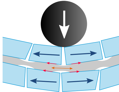
Figure I.8 Schematic of a cracked laminate in the “stretching” phase: displacement between two glass shards is approximated as a tensile deformation ( \leftarrow \rightarrow ). The interlayer ligament undergoes both stretching ( \leftrightarrow ) and delamination ( \rightarrow ) from the interface.
