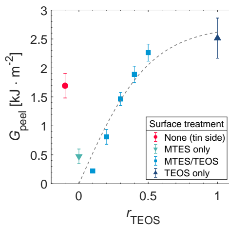
Figure III.2 Adhesive peel energy vs. TEOS content of the surface treatment. Peel tests at 50 \text{ mm} \cdot \text{min}^{-1} , 22^\circ\text{C} , 50%RH. The grey dashed line is a guide for the eye.
