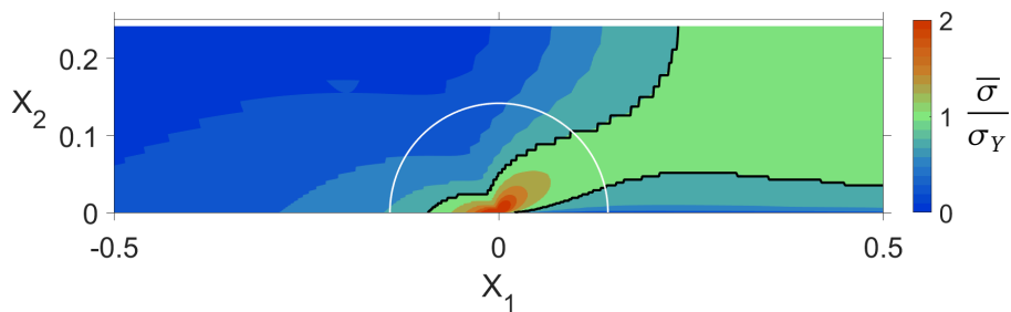
(c) \hat{\sigma}/\sigma_Y = 4
