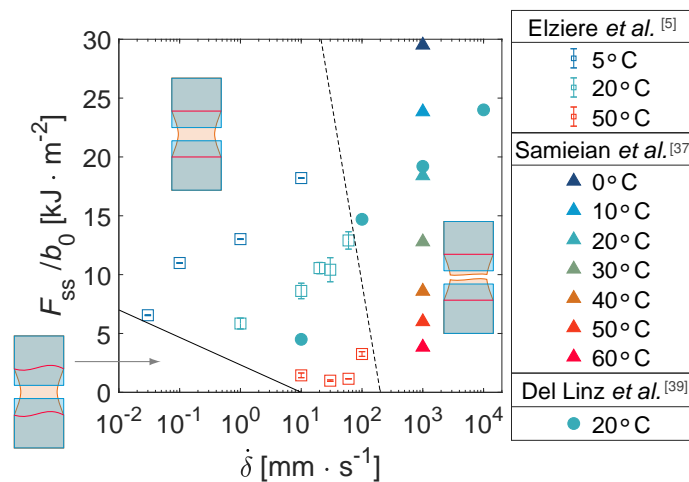
Figure I.9 Influence of traction velocity and temperature on the delamination force measured with the TCT-Test (PVB thickness = 0.76 mm) Solid line: empirical limit between unstable and steady delamination behaviors. Dashed line: empirical limit from steady behavior to rupture of the interlayer. [5,37,39]
