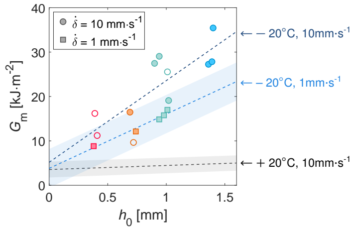
(c) Macroscopic work of fracture G_m vs. interlayer thickness. Shaded areas: 95% prediction bounds for the linear models. Prediction bounds are not drawn for the (-20^\circ\text{C}, 10\text{mm}\cdot\text{s}^{-1}) case.
