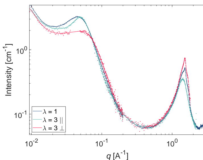
Figure IV.3 X-ray diffraction spectrum of EVA (combined SAXS and WAXS data). Isotropic integration for \lambda=1 . \lambda = 3 : azimuthal integration over a 30° angle parallel and perpendicular to the traction direction.
