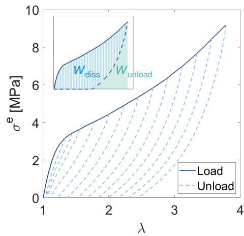
(a) Cyclic engineering stress vs. stretch curves. Intermediate re-loading curves are not shown.
