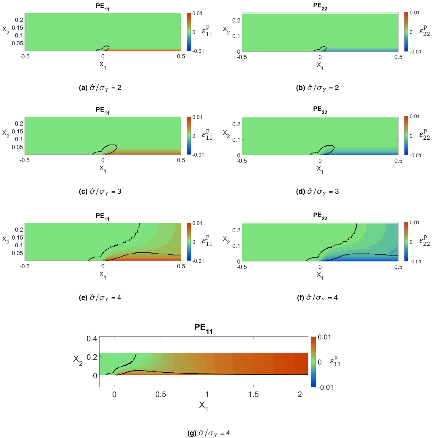
Figure VI.12 Plastic deformation in steady-state in converged step. Material parameters: E/\sigma_y = 50 , \nu = 0.45 , m = 3 and \nu = 1000 . The thick black lines indicates the active plastic zone size \bar{\sigma} = \sigma_Y .
