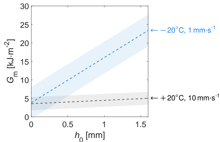
Figure VII.4 TCTT with EVA laminates: macroscopic work of fracture vs. interlayer thickness, at ambient temperature and close to the glass transition.
