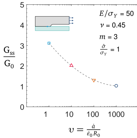
(c) Fracture energy vs. normalized crack velocity, in the case \hat{\sigma} = \sigma_Y .
