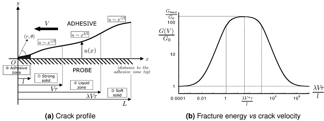
Figure I.12 De Gennes ’s “viscoelastic trumpet” model: the maximum value of G/G_0 is given by \lambda = \mu_0/\mu_\infty , the ratio of instantaneous modulus over relaxed modulus. From Saulnier et al. [51]
