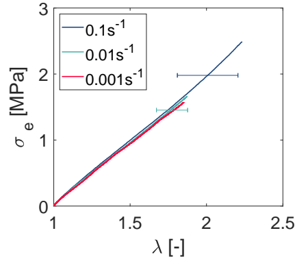
Figure IV.9 Tensile test to rupture for EVA at 80°C. The errorbars indicate the standard deviation of the strain at break (3 samples).
