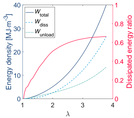
(b) Energy densities from tensile curves. Dissipated energy ratio = W_{\text{diss}} / W_{\text{total}} .
