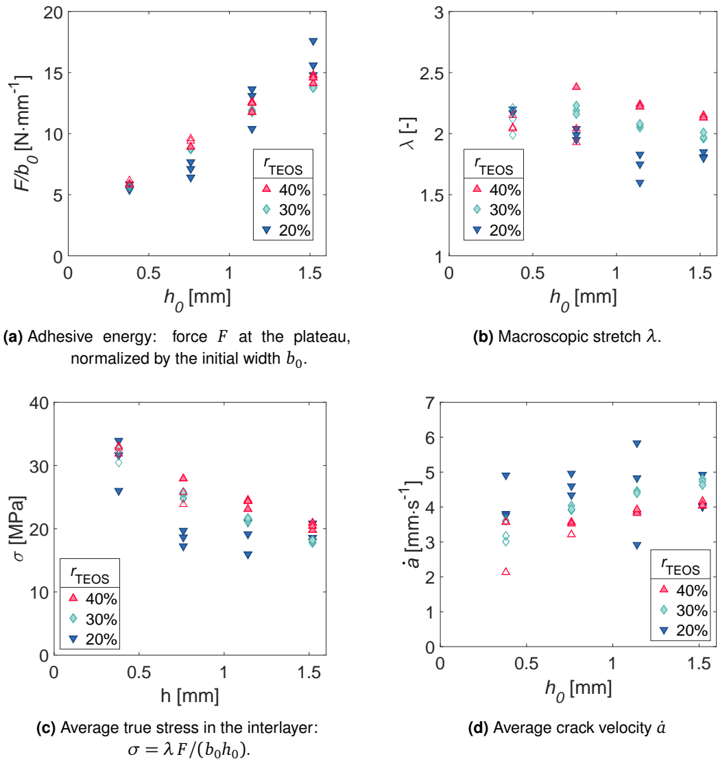
Figure III.9 Through Crack Tensile tests with varying PVB/glass adhesion. Filled symbols = steady-state delamination values. Open symbols = values before propagation arrest (interlayer rupture or asymmetric cracks)
