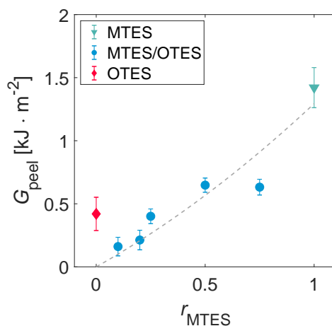
Figure V.3 Peel adherence of EVA vs. MTES content in MTES–OTES coatings. The grey dashed line only a guide for the eye.
