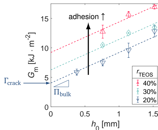
Figure VII.1 TCTT with PVB-laminated glass at various adhesion: macroscopic work of fracture vs. interlayer thickness.
