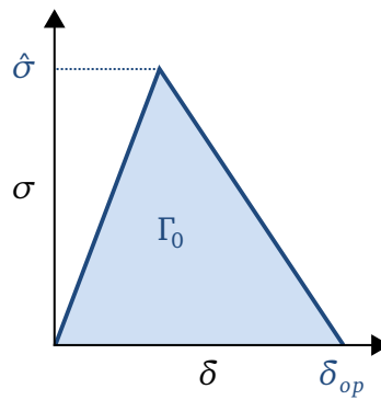
Figure I.11 Unidimensional bilinear traction-separation law for a cohesive zone model, characterized by a cohesive stress \hat{\sigma} and a separation energy \Gamma_0 .
