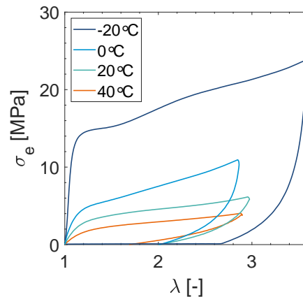
Figure IV.7 Engineering stress vs. stretch curves of EVA at the strain rate \dot{\lambda} = 0.5\text{s}^{-1} . Both Young's modulus and yield stress increased towards the glass transition ( T_g = -18^\circ\text{C} ).
