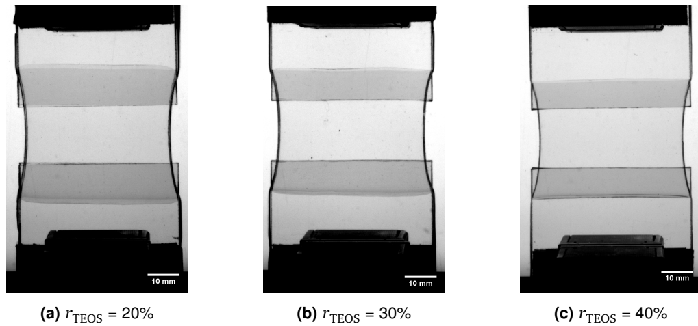
Figure III.3 TCTT: delamination of the PVB interlayer at \delta = 20 mm ( h_0 = 1.14 mm, \dot{\delta} = 10 mm·s -1 , T = 20^\circ\text{C} ).
