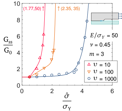
(b) Fracture energy vs. cohesive stress: effect of the normalized crack velocity v .
