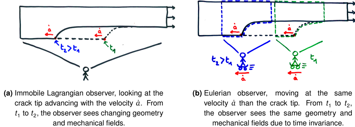
Figure VI.5 Illustration of the Lagrangian vs. Eulerian frameworks in a steady-state regime.
