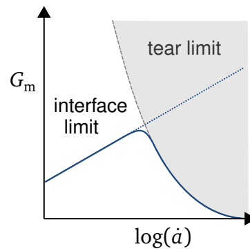
Figure VII.3 Velocity limit for the macroscopic work of fracture
