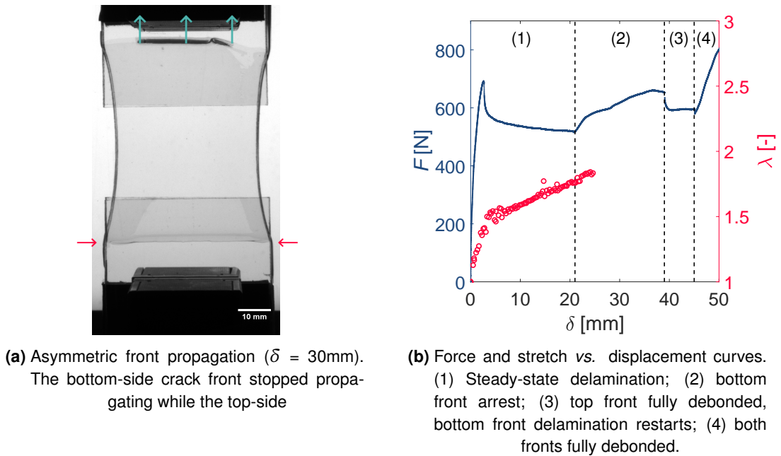
Figure III.8 Crack arrest phenomenon and asymmetric propagation at low adhesion and thick interlayer ( r_{\text{TEOS}} = 20\% , h_0 = 1.14 mm).
