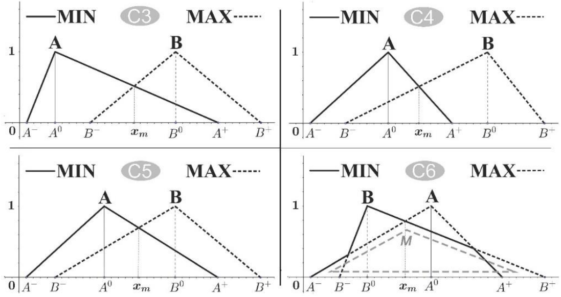
Fig. 5-18. Topological Representation of the Situation 3: overlapping cases
