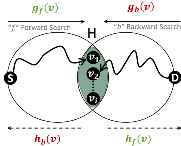
Fig. 6-6. Bidirectional Time-Dependent Fastest Path problem (BTFP)
