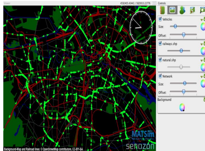
Fig. 3-13 Interface of simulation of MATSim by Senozon
