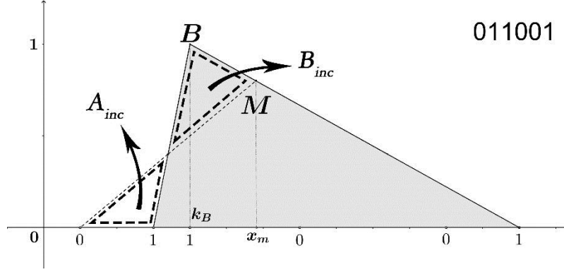
Fig. 5-20. The degree of inclusion in \text{MIN}(A, B)
