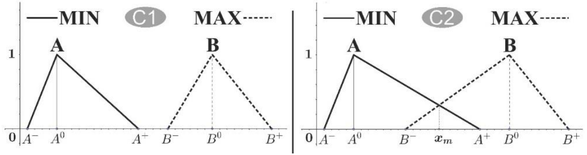
Fig. 5-17. Topological Representation of the Situation 1 & 2: Disjoint & Weak cases
