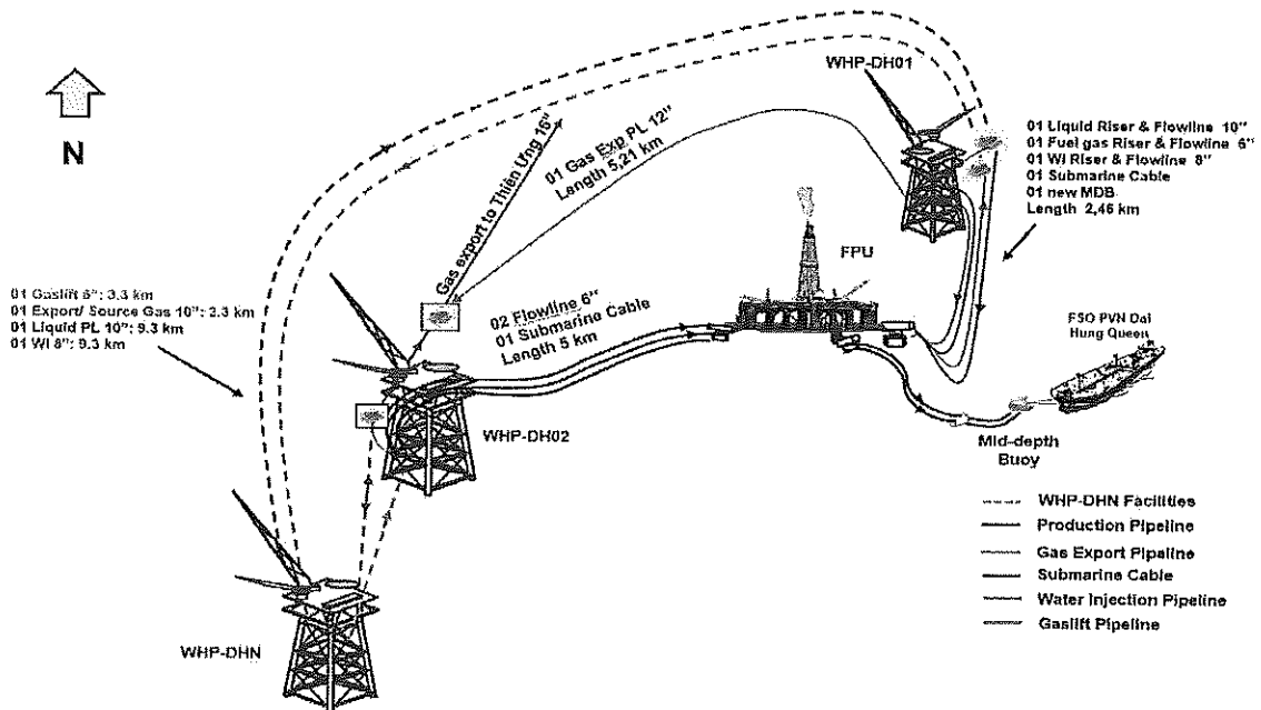
Figure 1.1: DAI HUNG FIELD FACILITIES: FPU + FSO + WHP-DH01+ WHP-DH02+WHP DHN
