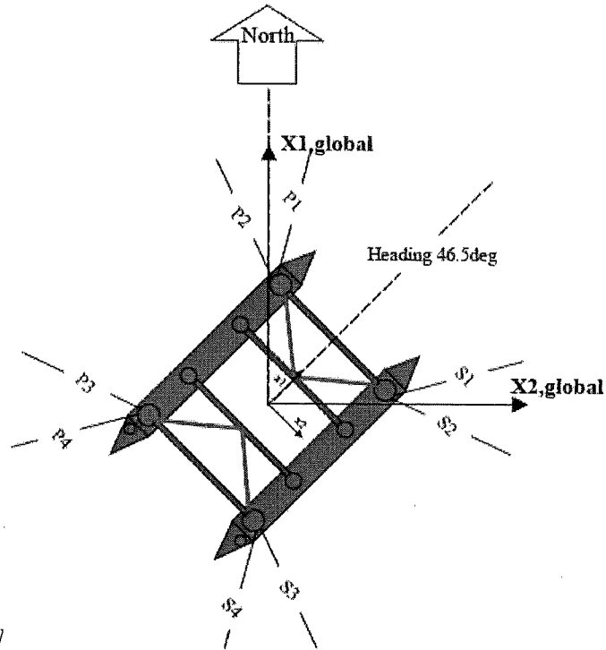
Figure 5: Layout of position & Mooring System of Dai hung 01 FPU
