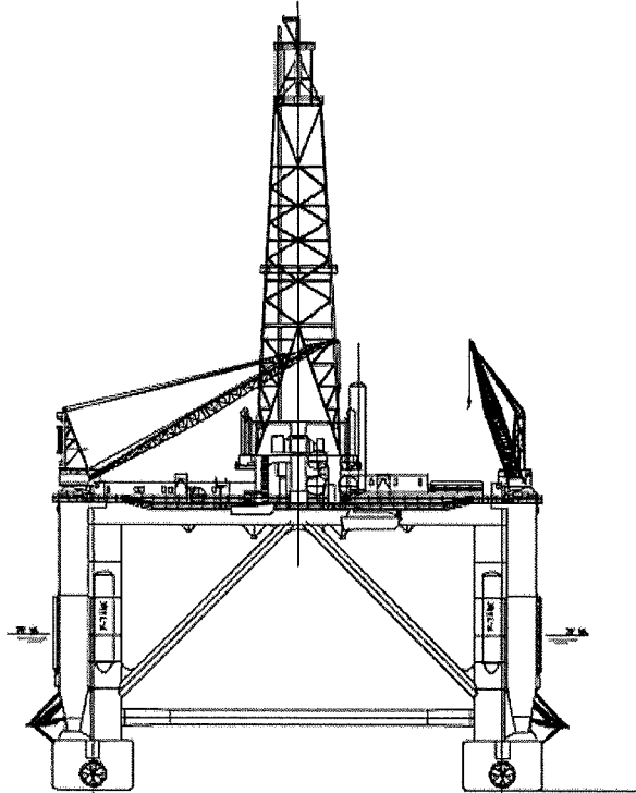
Figure 2: Dai Hung 01 stern view
