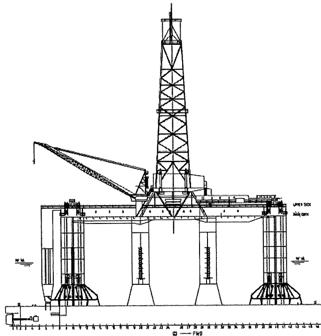
Figure 3: Dai Hung 01 starboard view
