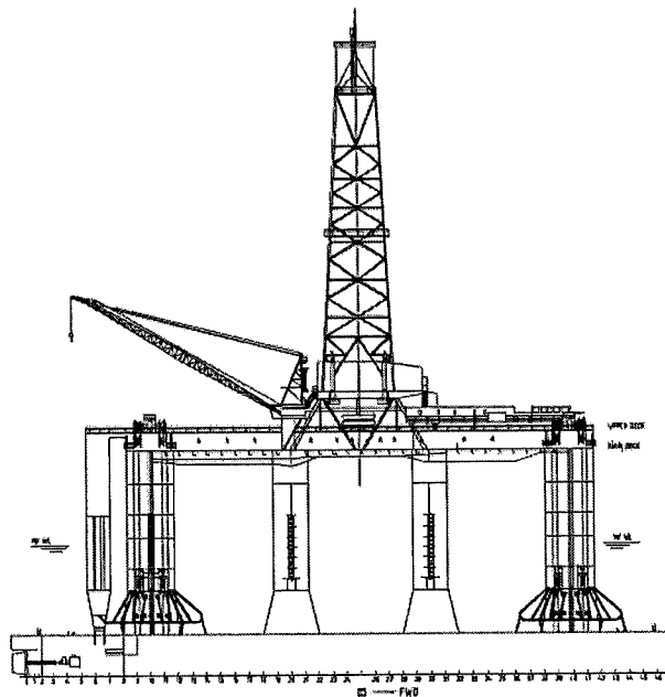
Figure 1: FPU DH-01
